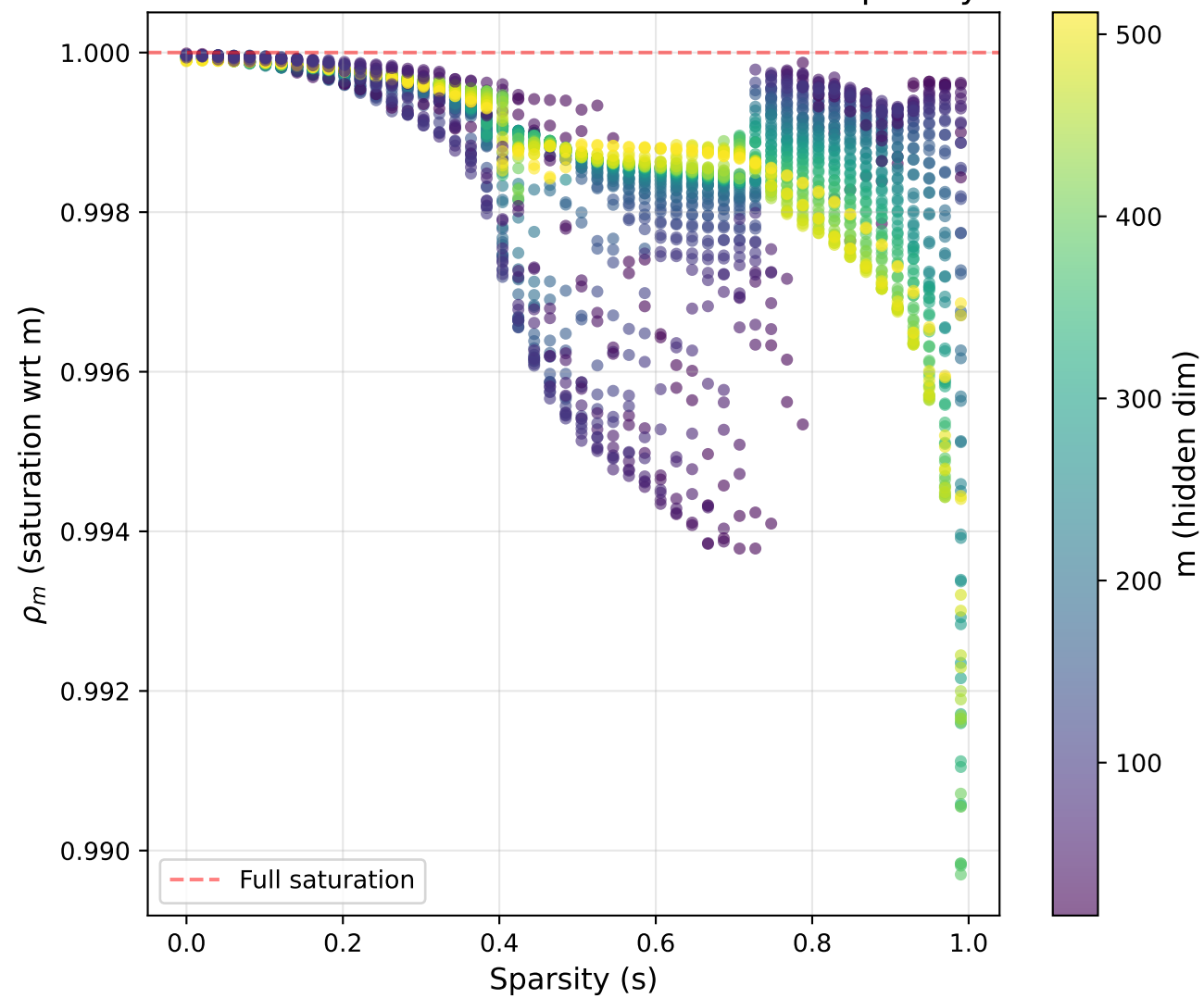
Panel 3: Saturation wrt Hidden Dim vs Sparsity
