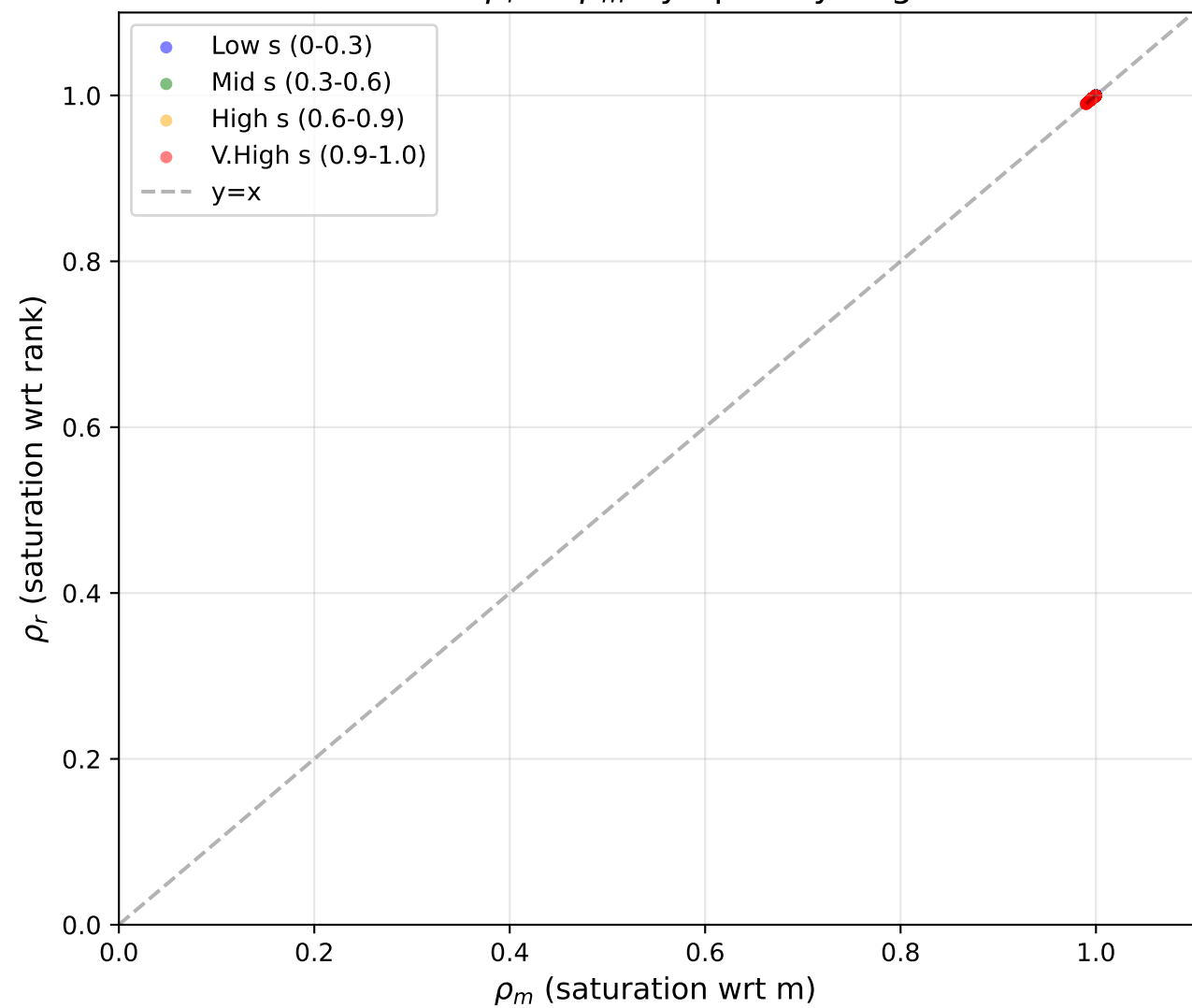
Panel 4: \rho_r vs \rho_m by Sparsity Regime
