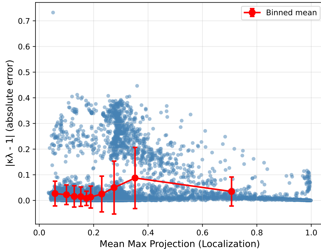
Conjecture Error vs Localization
