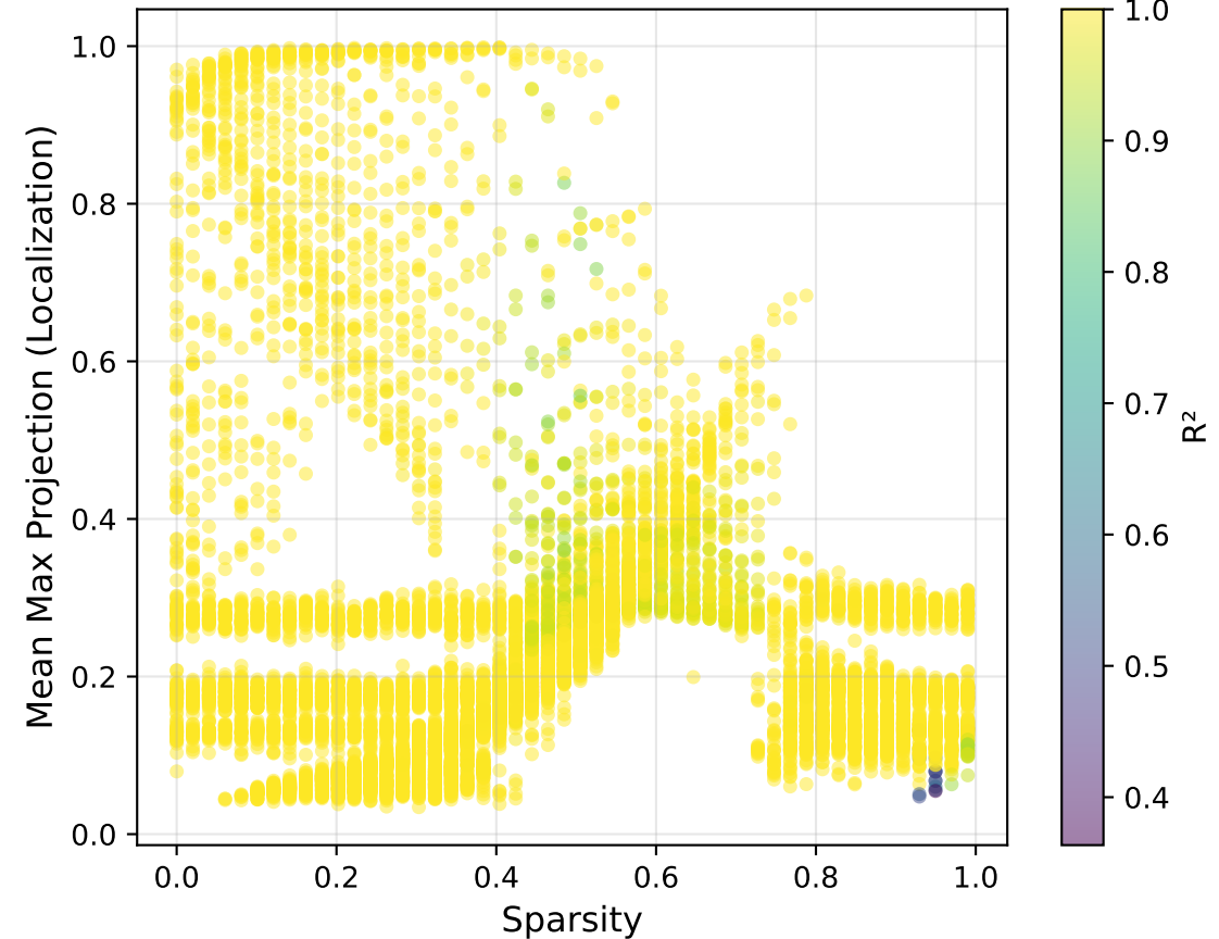
Localization vs Sparsity
