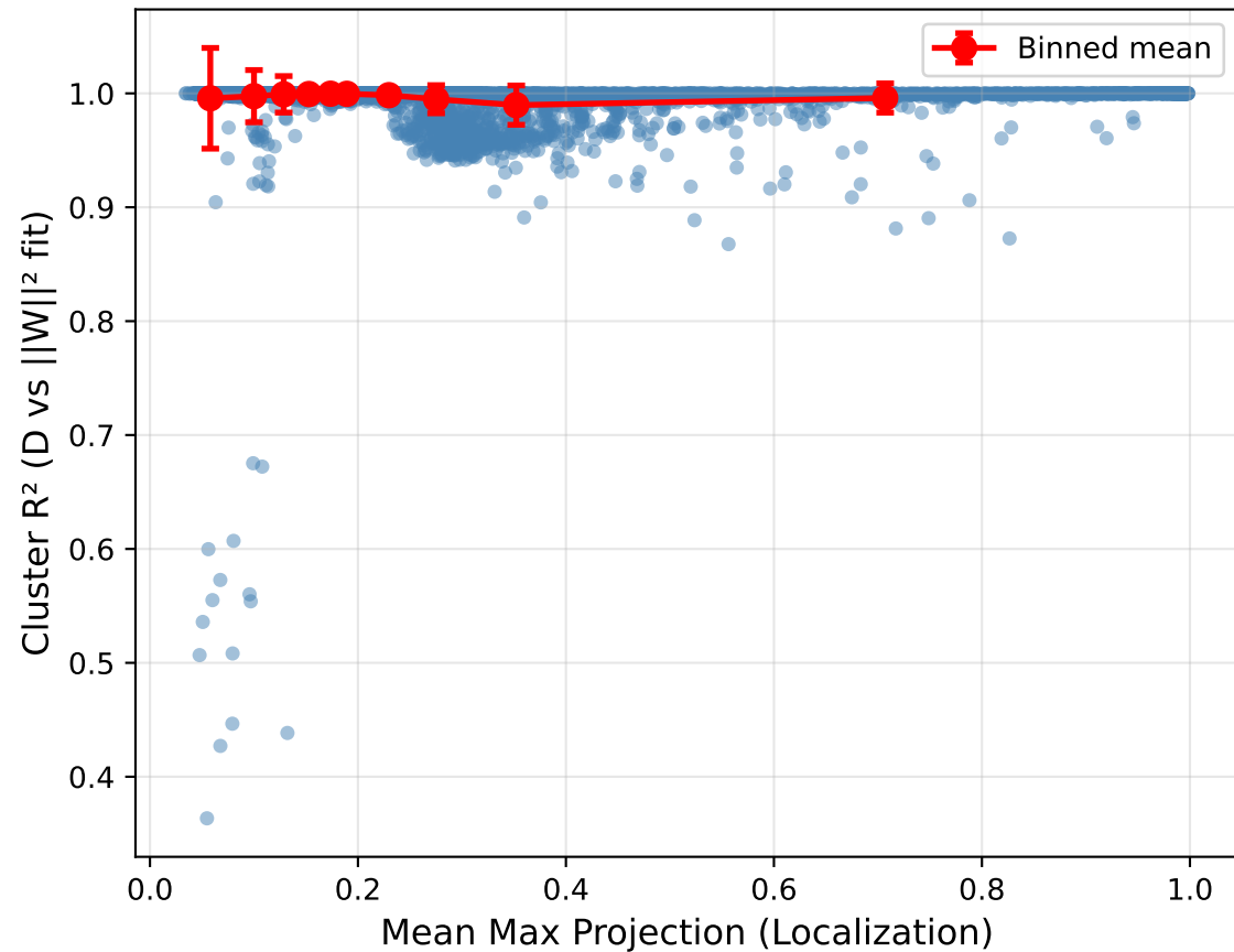
Fit Quality vs Localization
