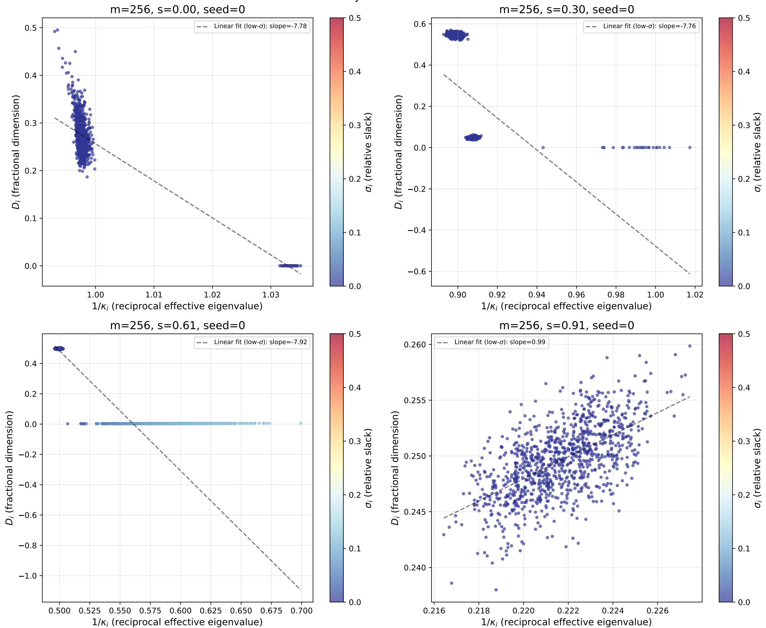
Plot C: Eigenvalue-Reciprocal Relationship Colored by Delocalization Slack
