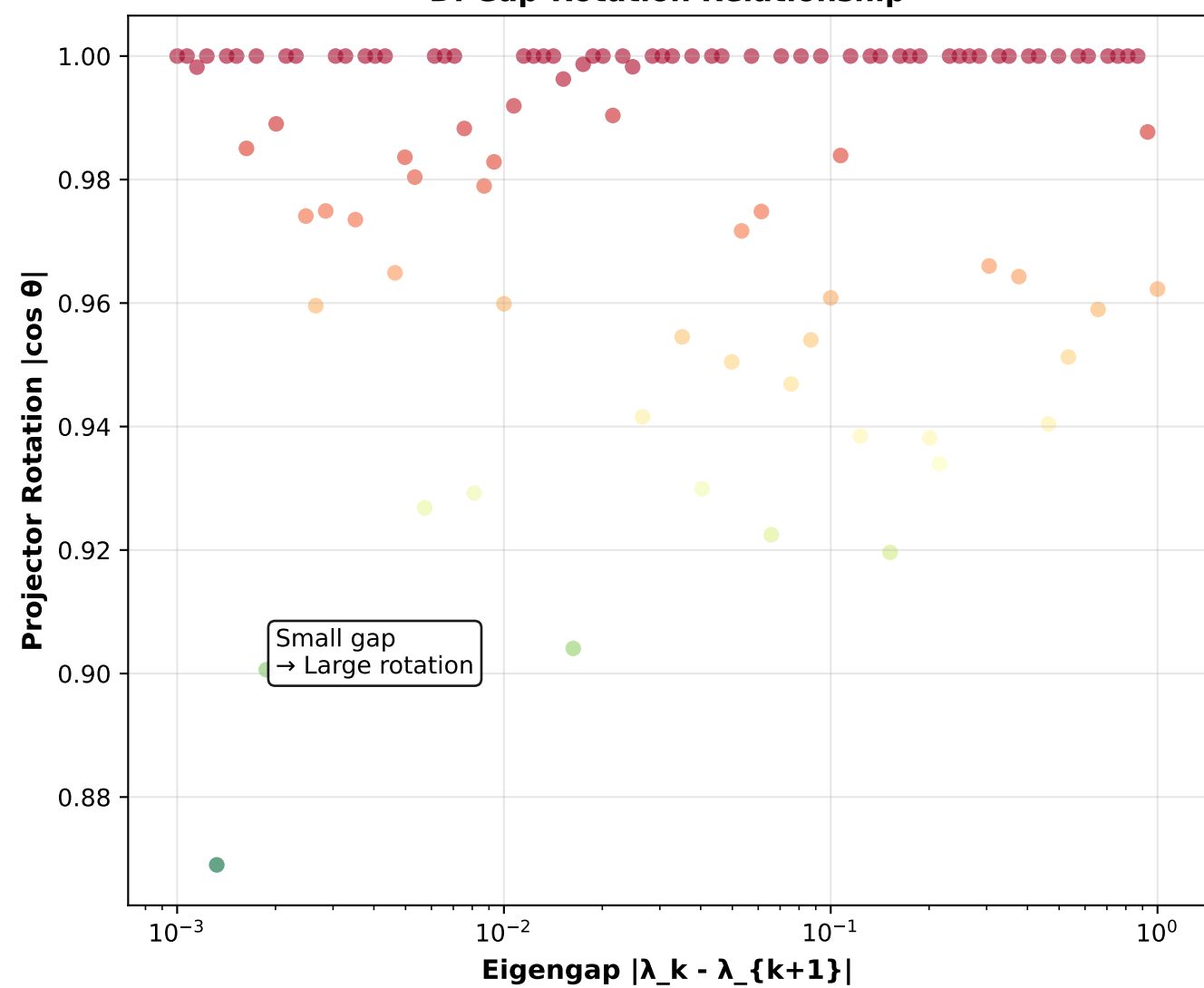
D. Gap-Rotation Relationship
