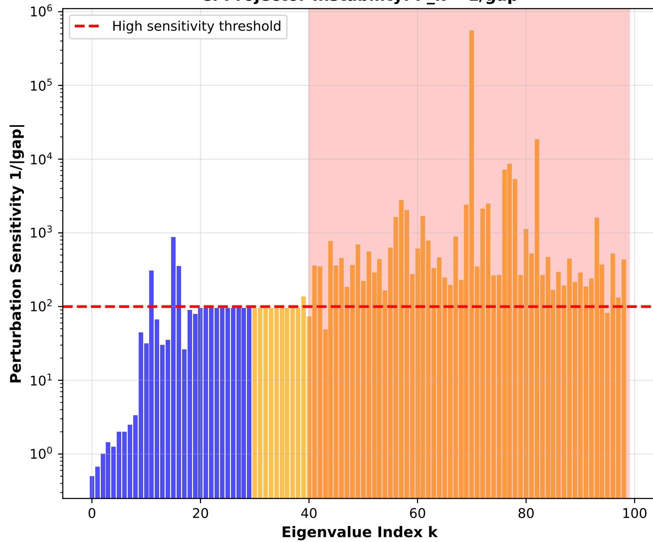
C. Projector Instability: \dot{P}_k \propto 1/\text{gap}
