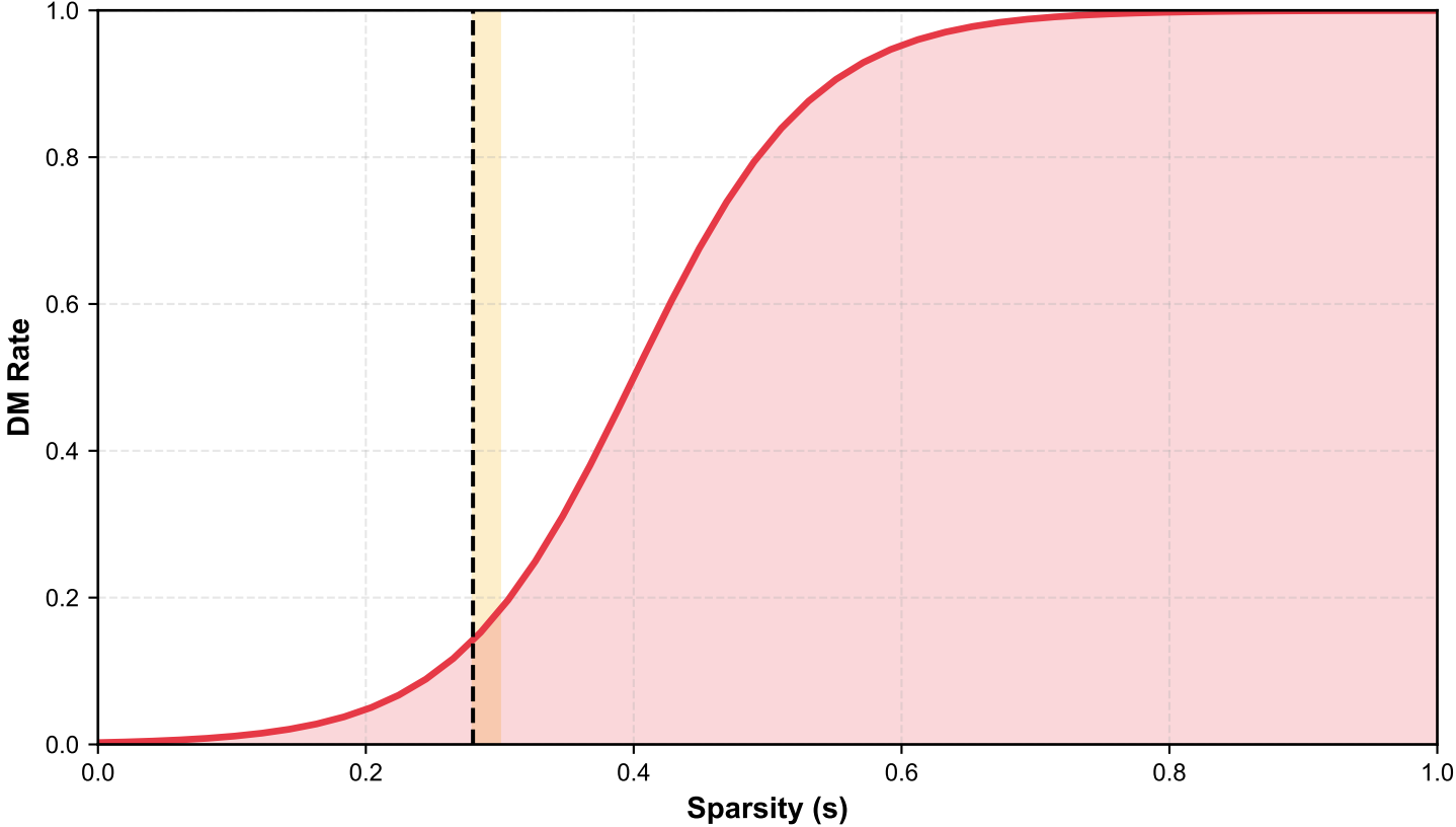
B. Phase Transition at s \approx 0.28
