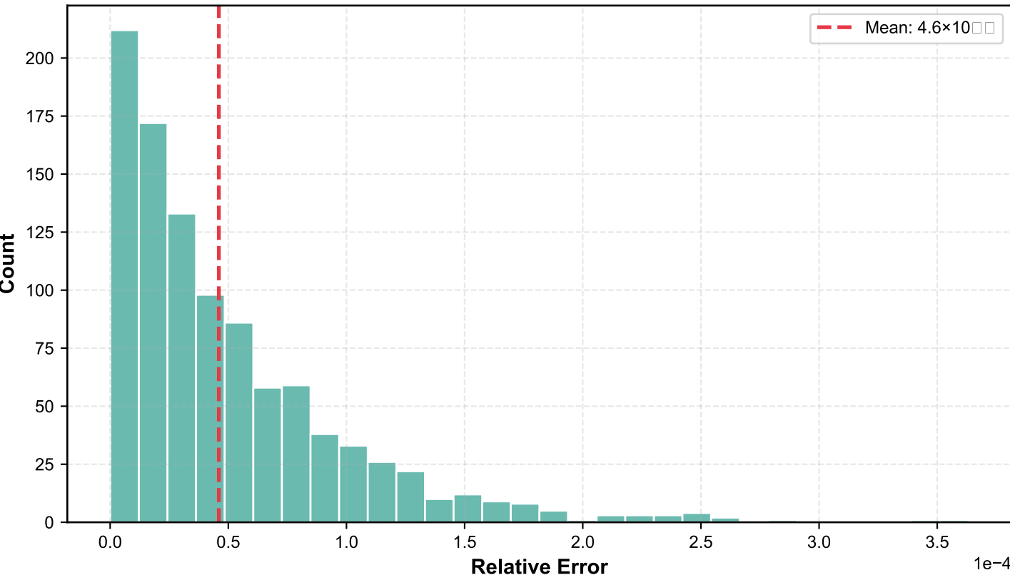
C. Spectral Measure \kappa = \sum p_i \lambda_i Validation
