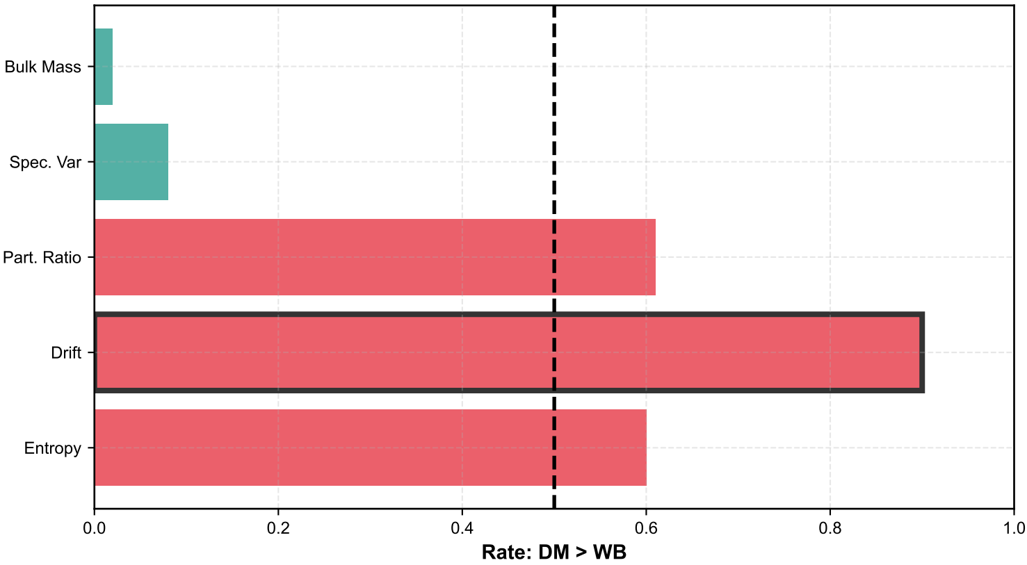
D. Drift: Primary DM Discriminator
