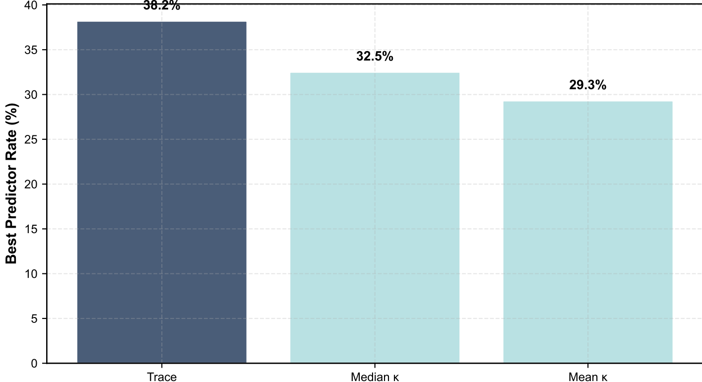
G. Trace Best Predicts \alpha(t)
