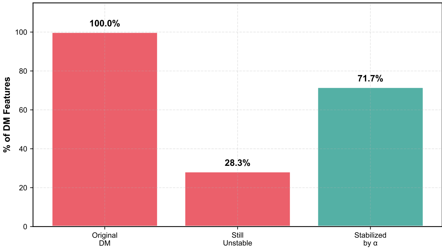
F. \alpha -Normalization Stabilizes 72% of DM
