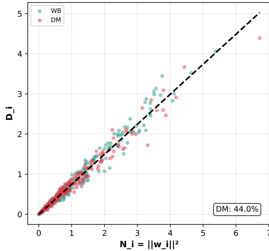
Late Transition R^2 = 0.971, \alpha = 0.75
