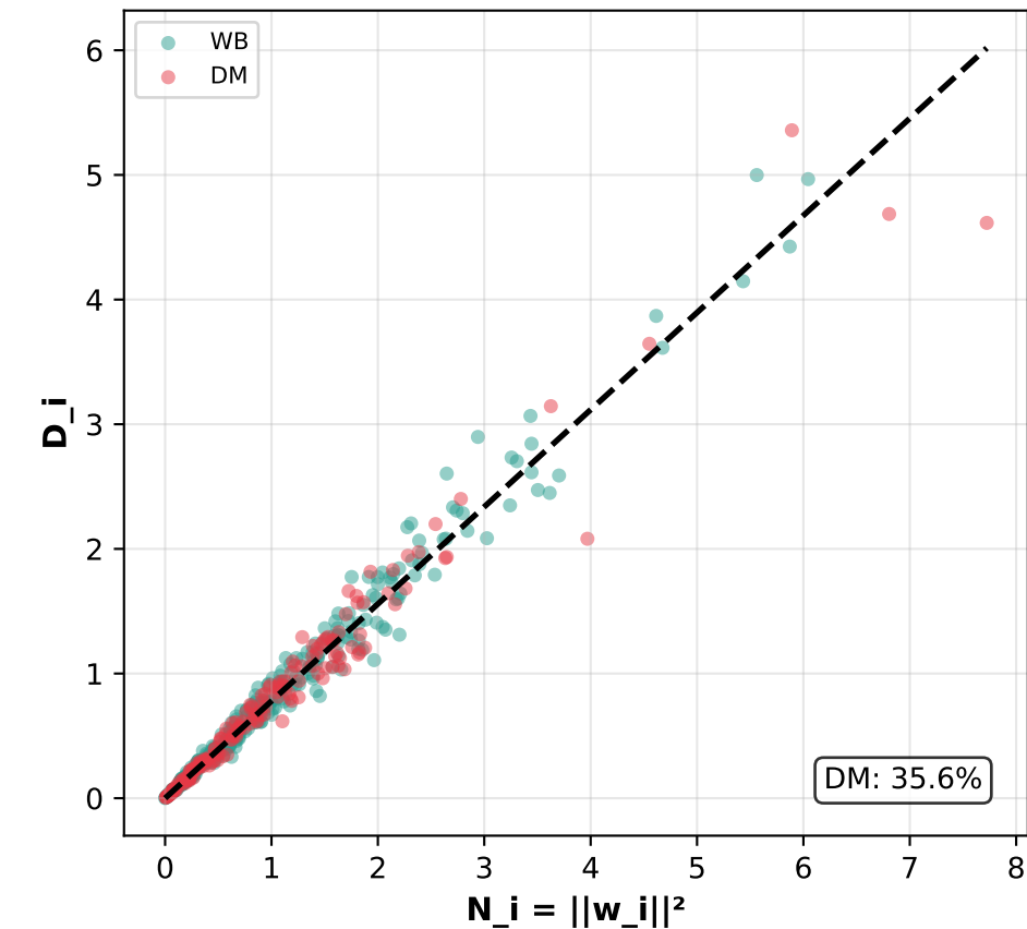
Highly Delocalized R^2 = 0.876, \alpha = 0.61
