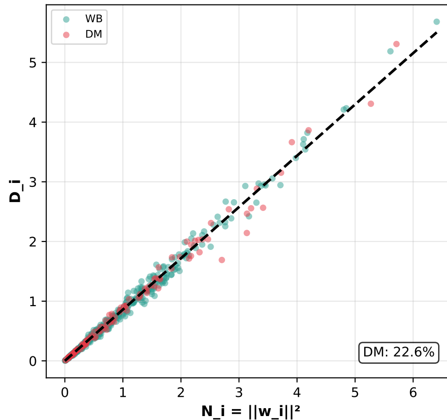
Delocalized R^2 = 0.931, \alpha = 0.71
