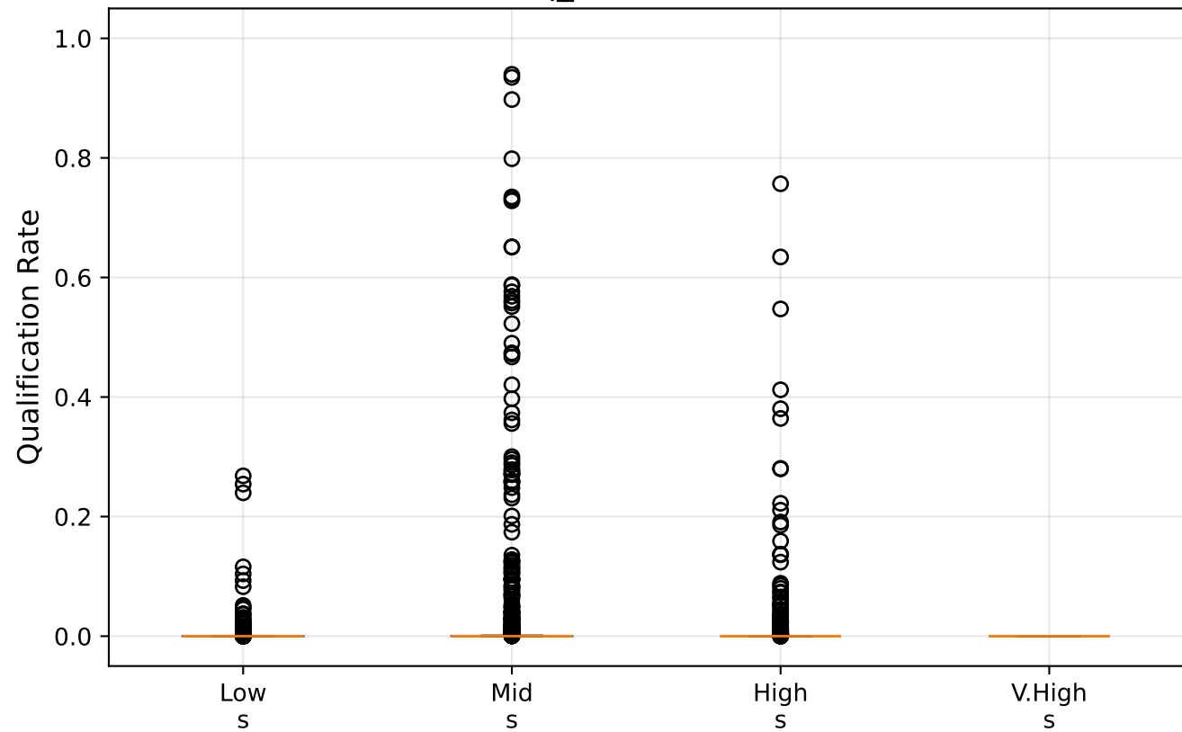
Qualification Rate Distribution by Sparsity Regime ( q_{\text{bin}} \geq 0.9 )
