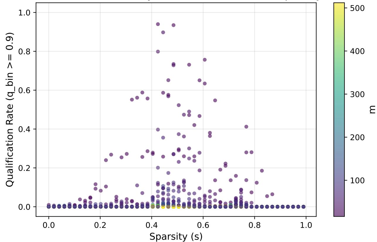
Fraction of Confidently Localized Features vs Sparsity
