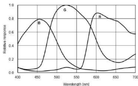
SC1200C量子曲线
