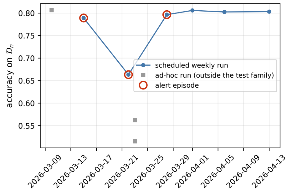
gpt-4.1-mini: detected degradation and self-recovery
