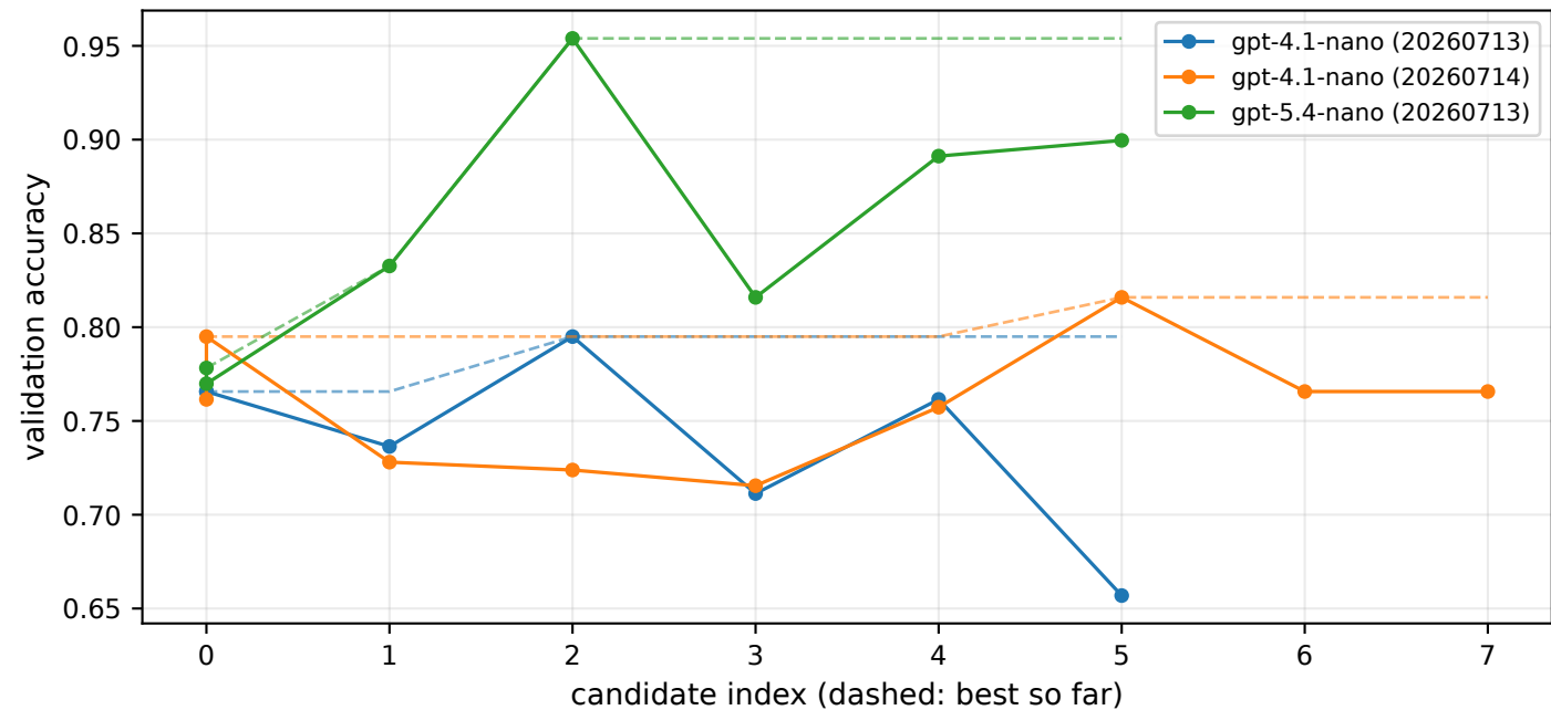
Prompt search trajectories on the 239-item validation split
