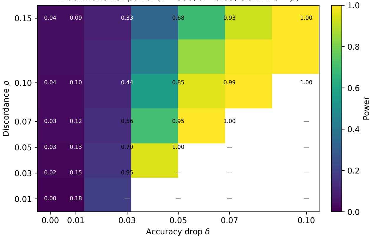
Exact McNemar power ( n = 300 , \alpha = 0.05 ; blank if \delta > \rho )
