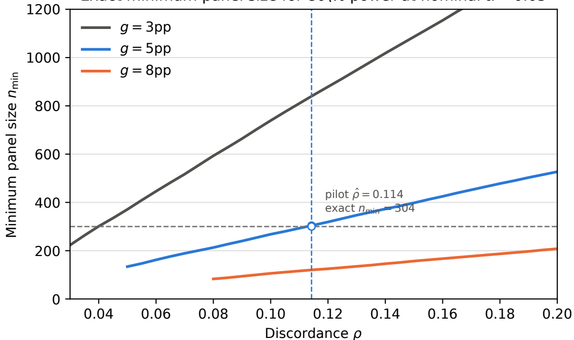
Exact minimum panel size for 80\% power at nominal \alpha = 0.05
