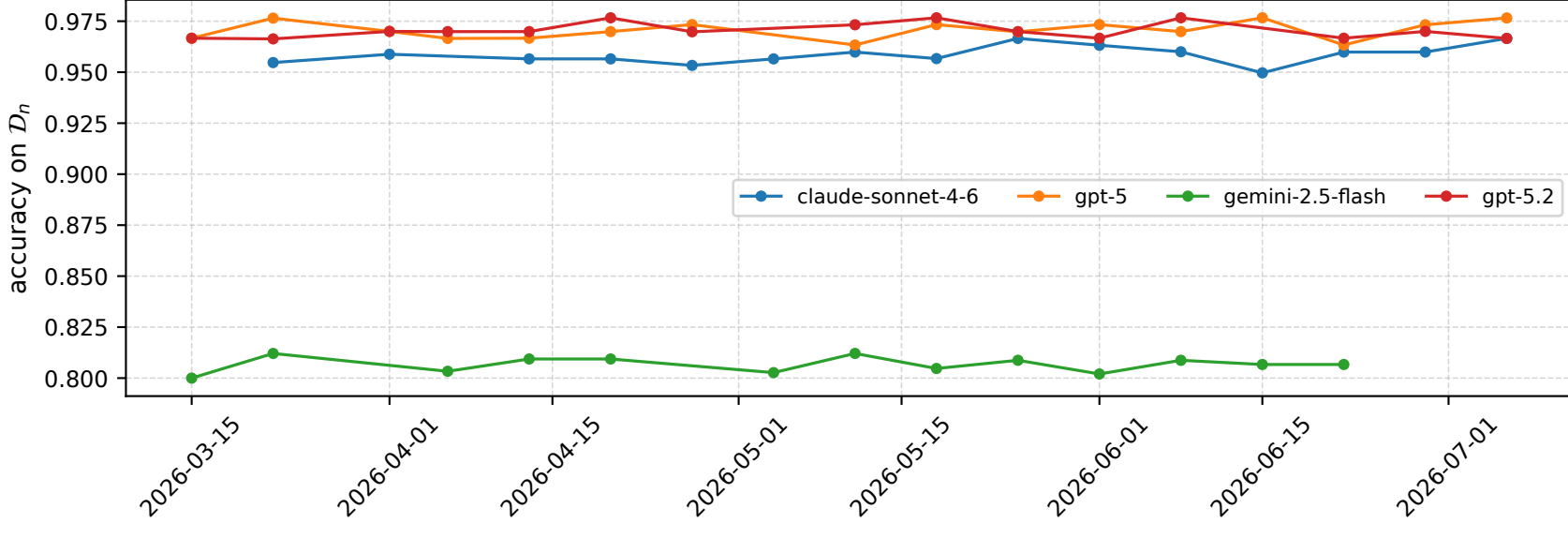
Weekly panel accuracy, the four most stable models
