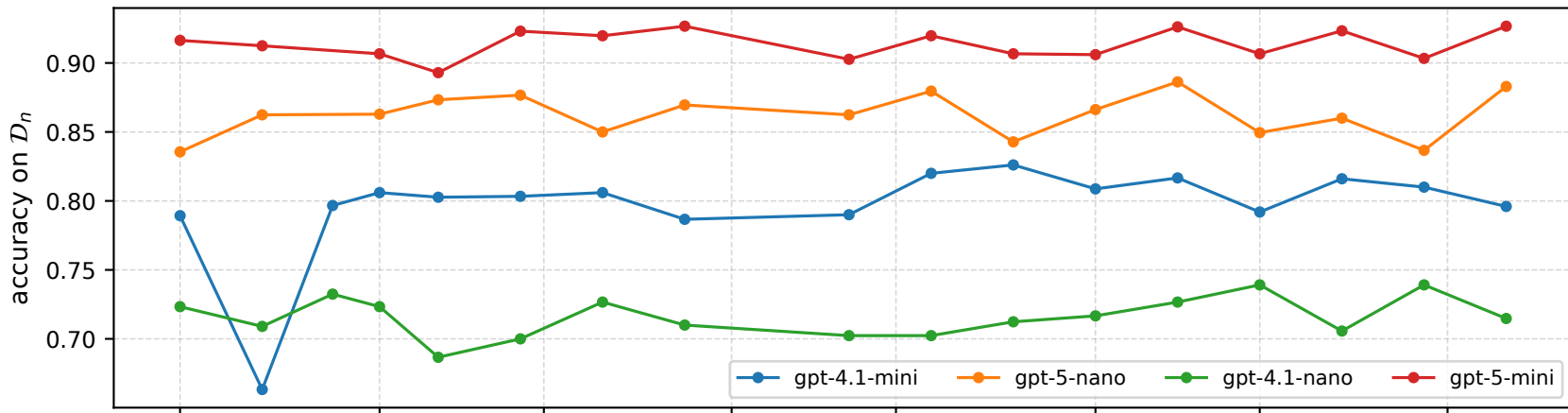
Weekly panel accuracy, the four most stable models
