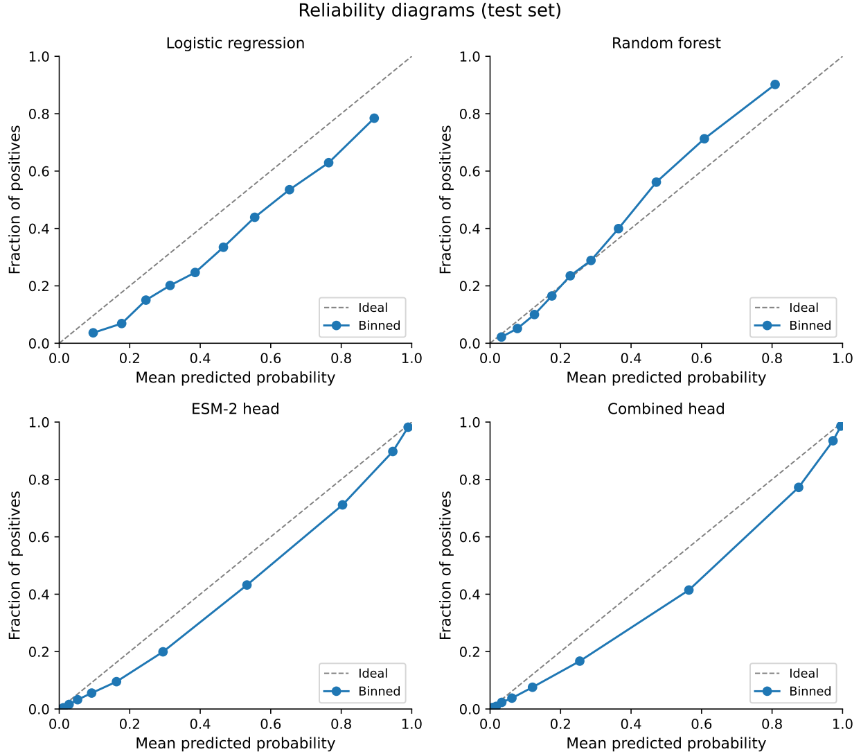
Figure A1: Reliability diagrams. Calibration curves for the four in-house scorers (10 quantile bins). Points should hug the diagonal under perfect calibration.
