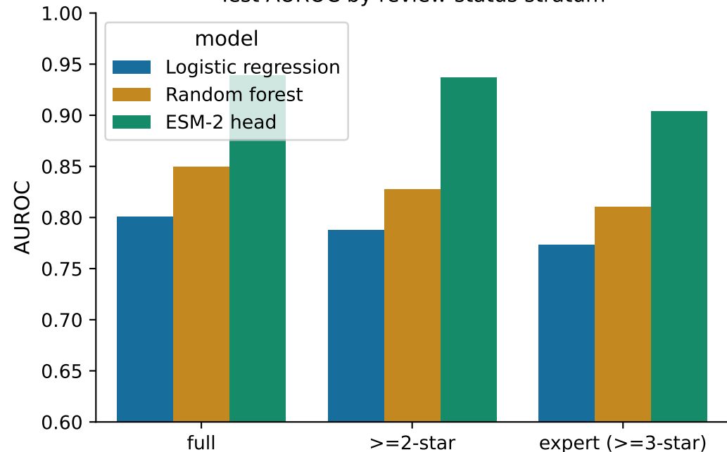
Test AUROC by review-status stratum
