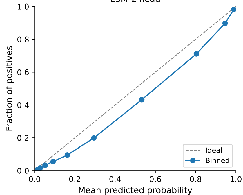
ESM-2 head
