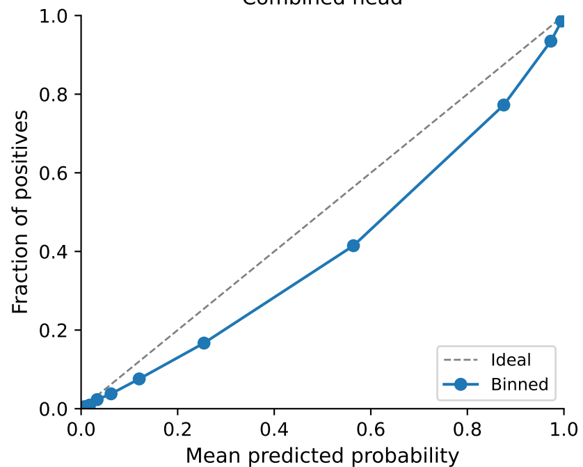
Combined head
