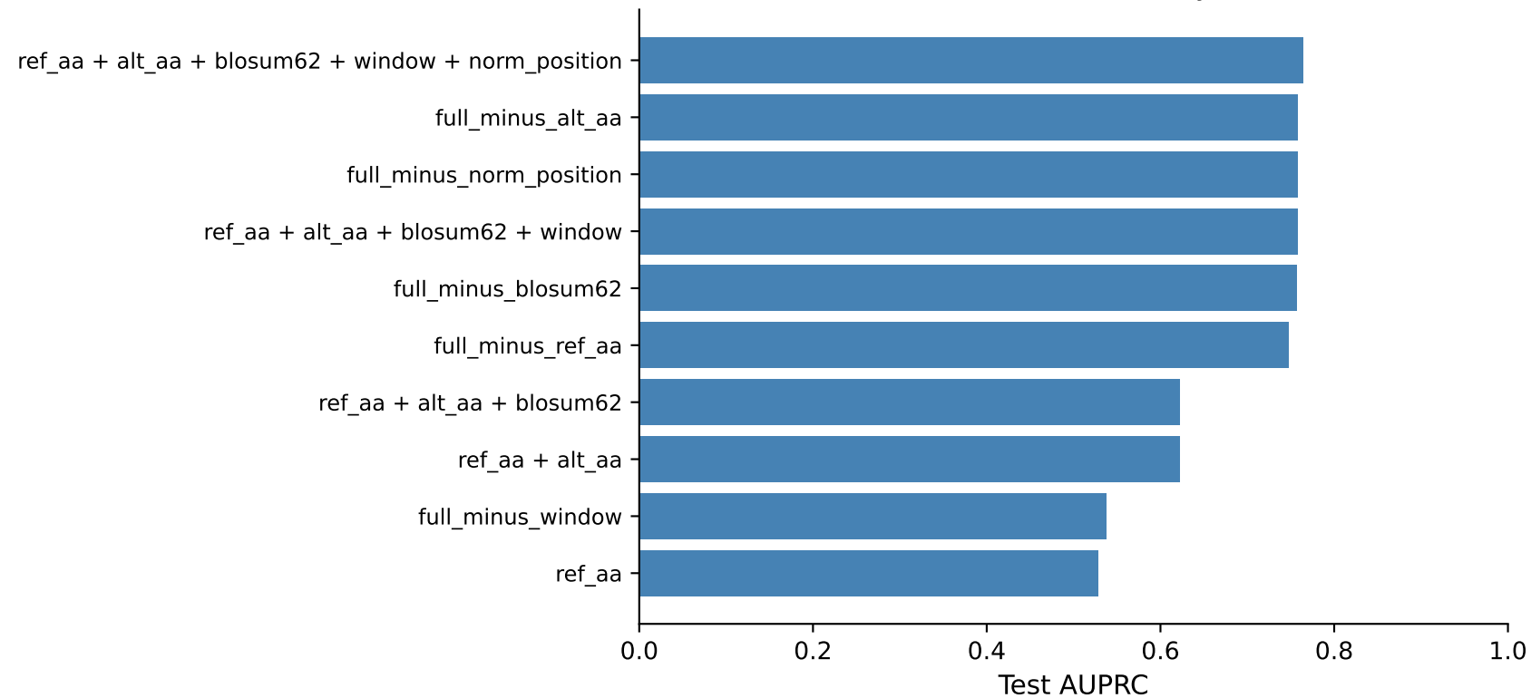
Random forest feature-family ablation
