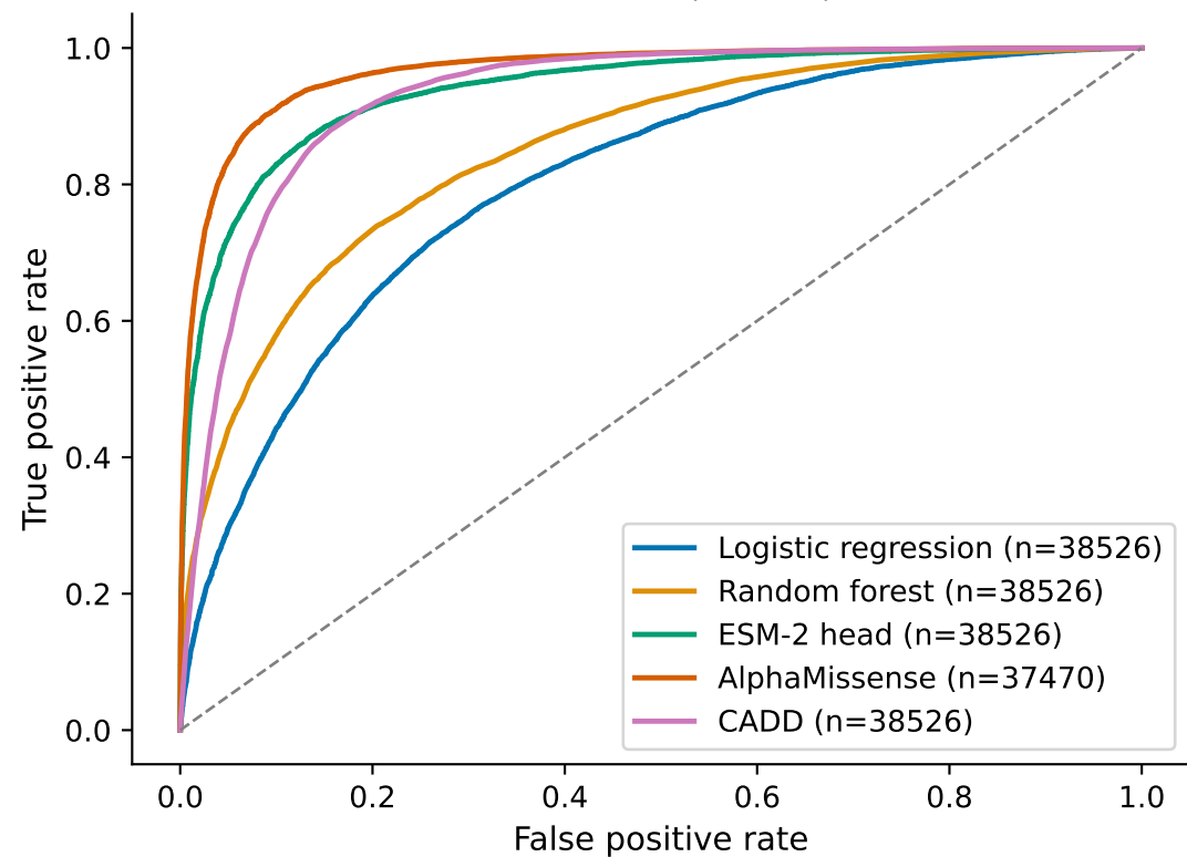
ROC curves (test set)
