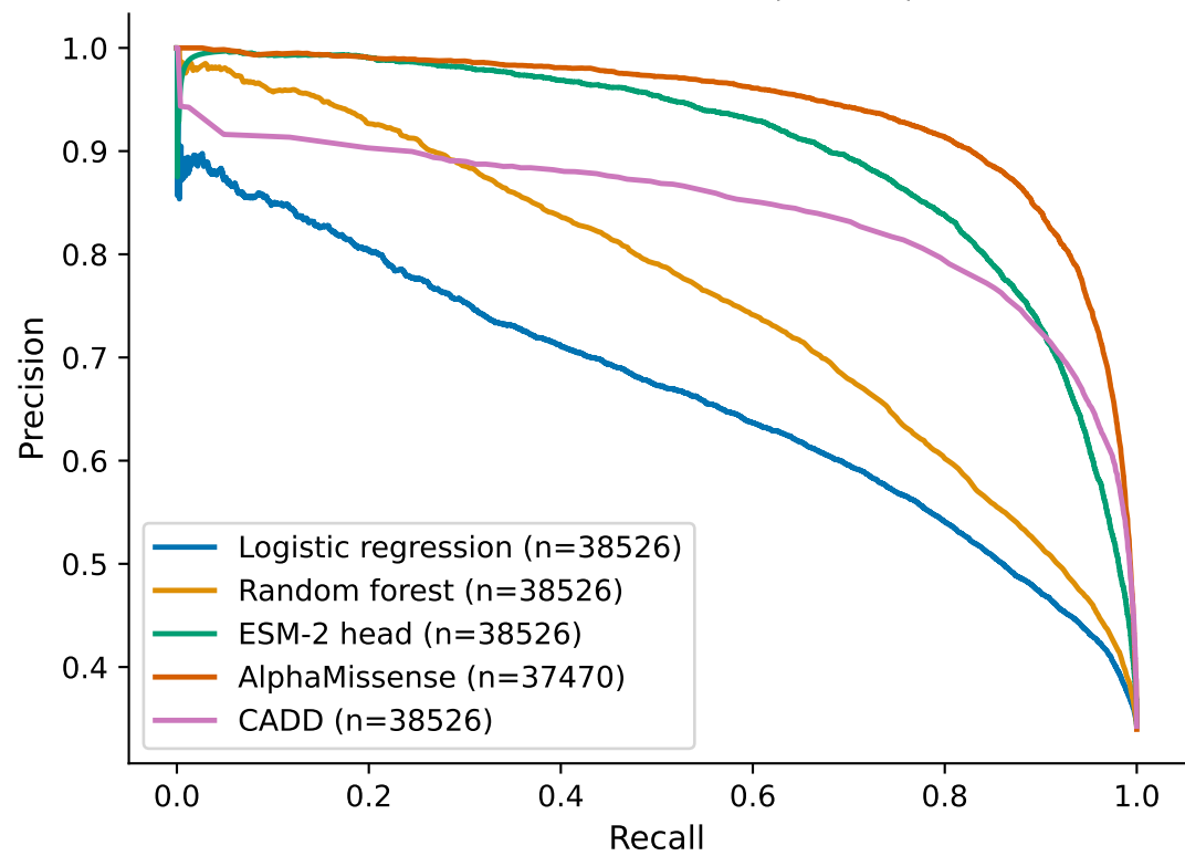
Precision-recall curves (test set)
