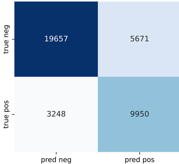
Random forest threshold=0.316, n=38526
