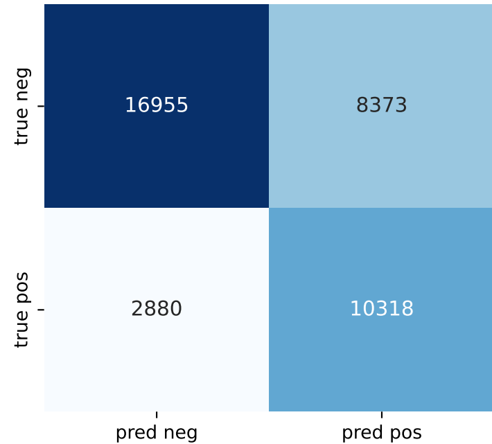
Logistic regression threshold=0.436, n=38526
