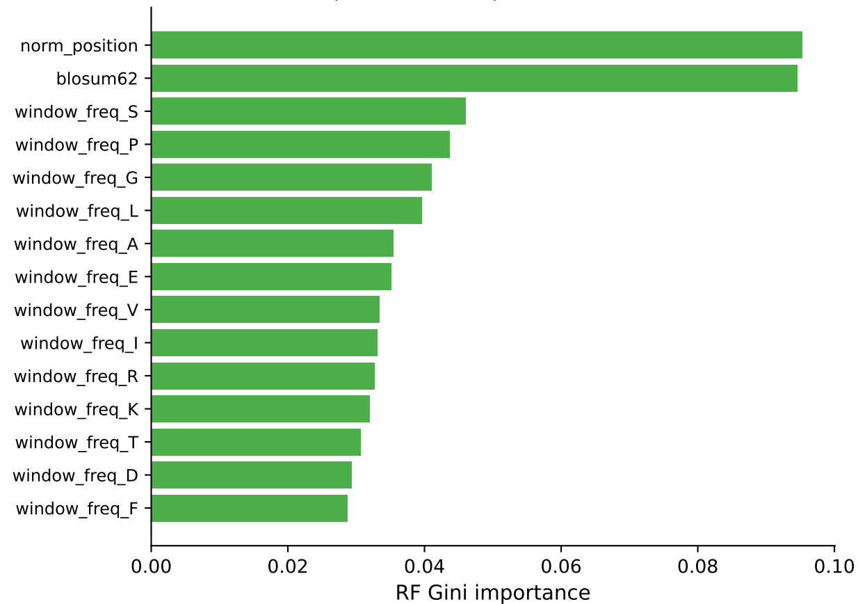
Top-15 RF Gini-importance features
