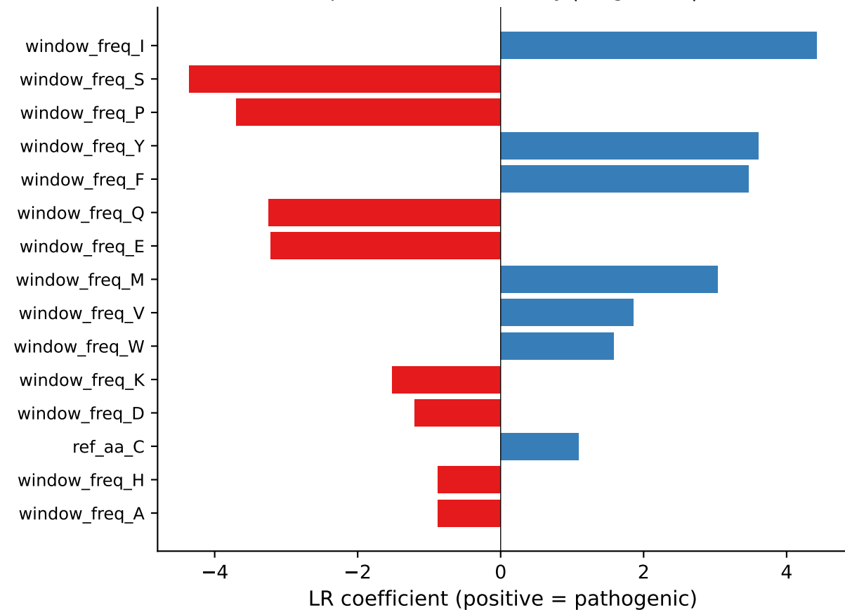
Top-15 LR coefficients by |magnitude|
