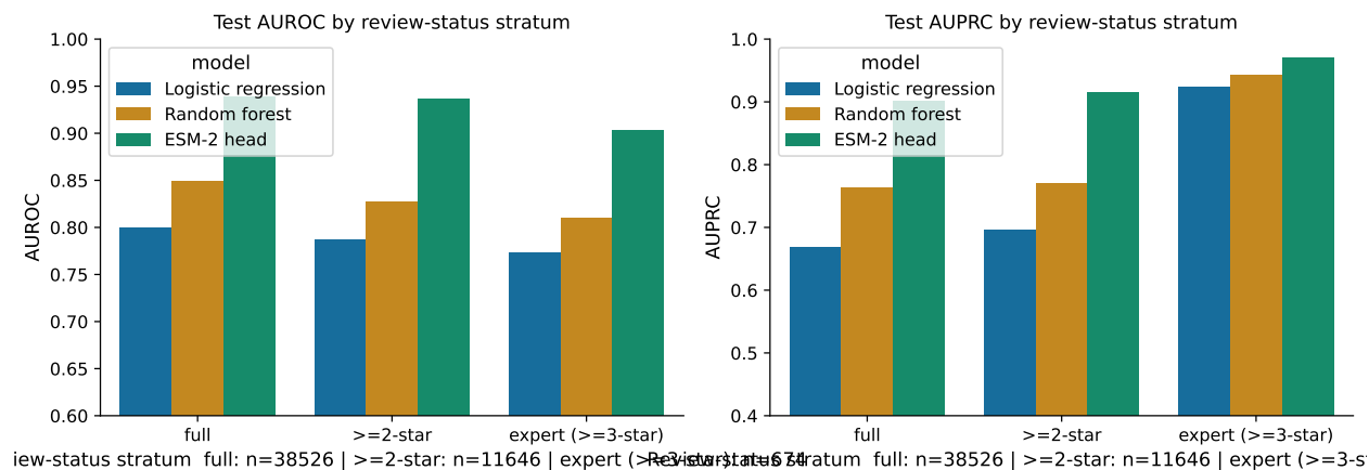
Figure 10: Figure 8 / Review-status sensitivity. Test AUROC and AUPRC stratified by ClinVar review-status confidence: full retained set, \geq 2 -star (criteria, multiple submitters, no conflicts), and expert ( \geq 3 -star: reviewed by expert panel or practice guideline). Conclusions hold across strata; the small expert-only stratum is more variable.
