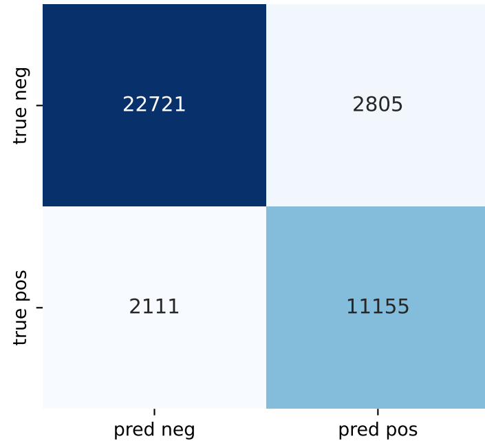
ESM-2 head threshold=0.499, n=38792
