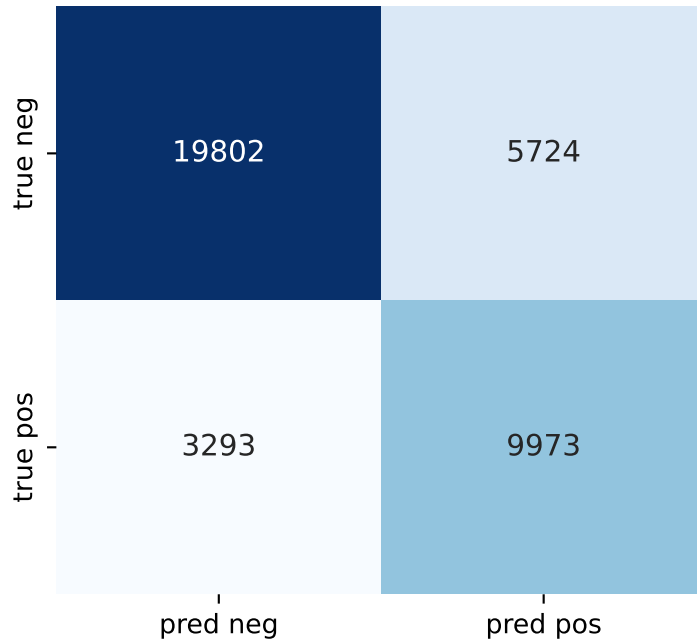
Random forest threshold=0.316, n=38792
