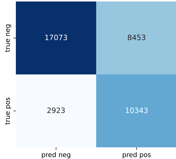
Logistic regression threshold=0.436, n=38792
