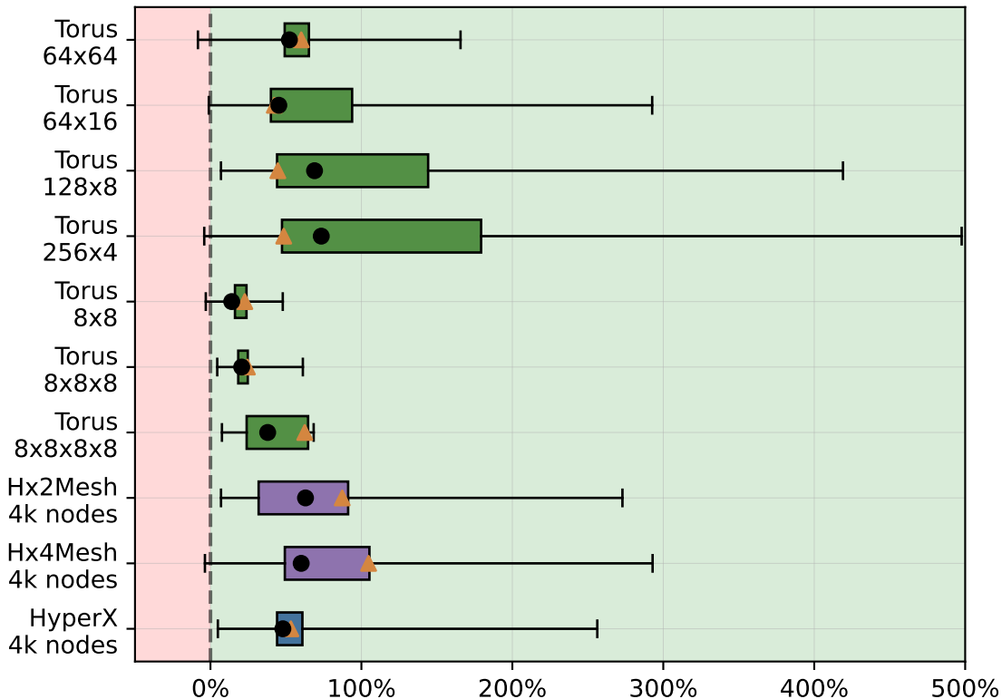
Goodput Gain vs. Best Known Algo. for Allreduce \leq 256\text{MiB}
