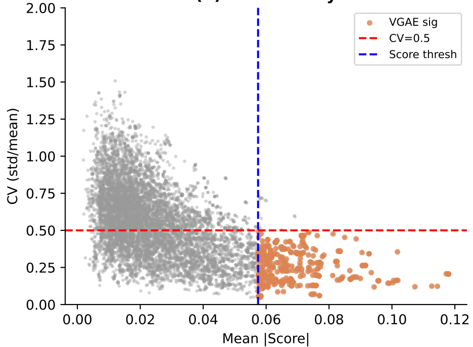
(b) Consistency
