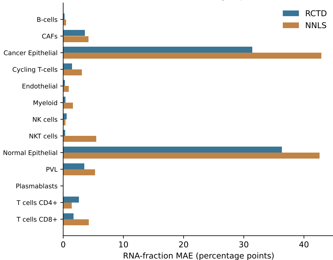
Factorial mixtures | depth 1
