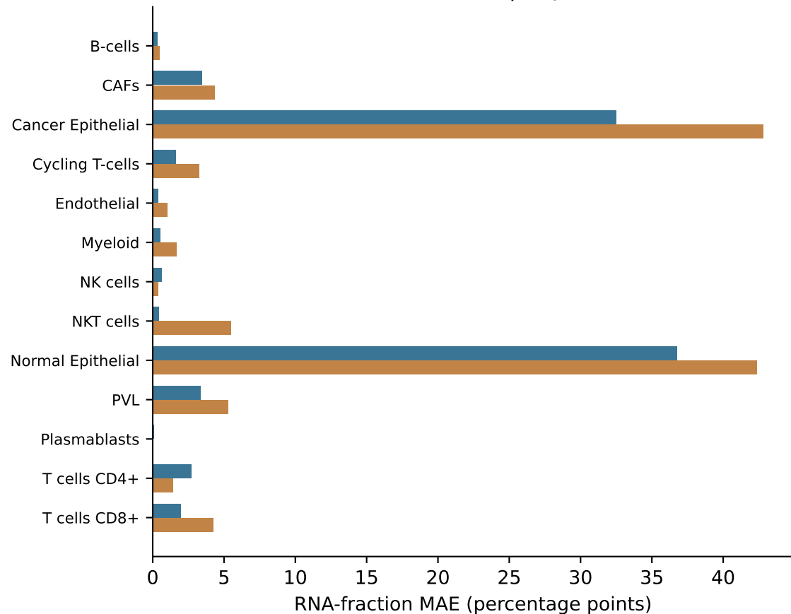
Factorial mixtures | depth 0.25
