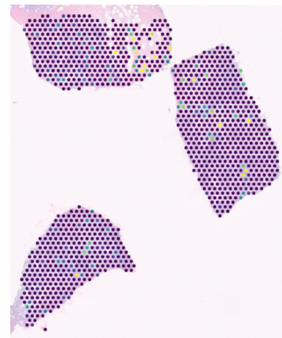
CID44971 | NK cells
