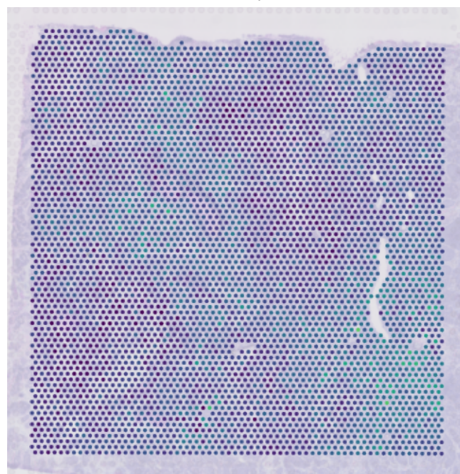
T relative weight (%) | shared scale 1142243F | TNBC
