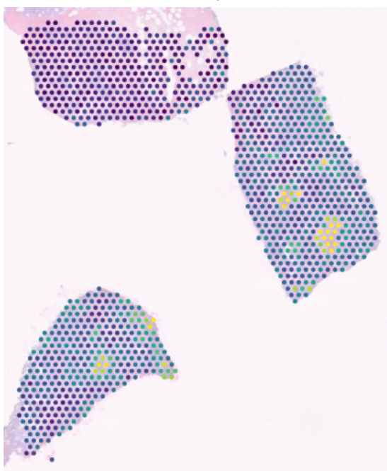
T relative weight (%) | shared scale CID44971 | TNBC
