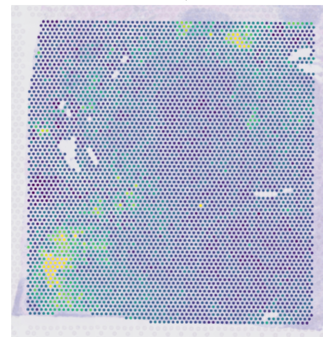
T relative weight (%) | shared scale 1160920F | TNBC
