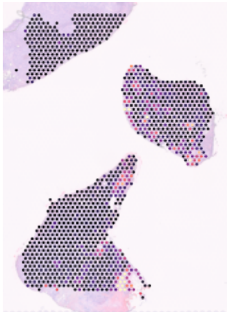
B T cells CD8+
