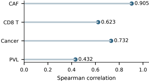
F Marker-expression concordance
