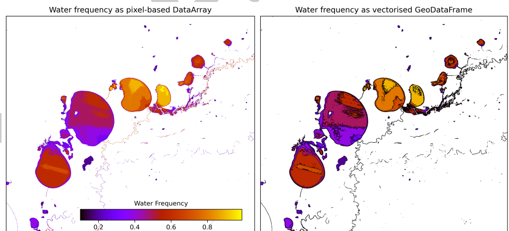
Figure 2: dea-tools enables easy transitions between xarray and geopandas with the xr_rasterize and xr_vectorize functions. Location is the Menindee Lakes, New South Wales
