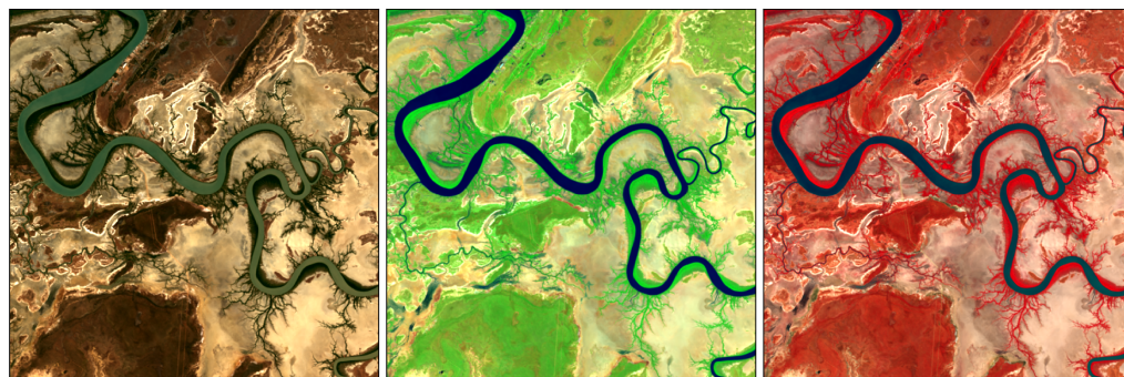
Figure 2: True and false colour composites generated with the dea-tools.plotting.rgb function, using DEA annual GeoMAD composite images from 2024.
