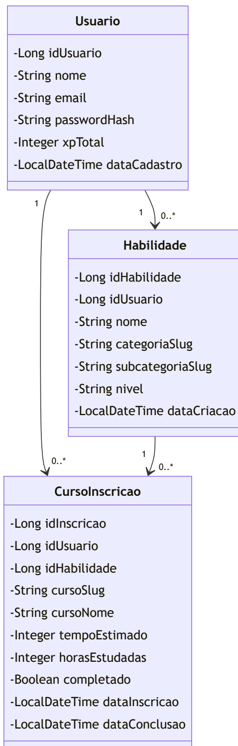
Diagrama de Classes UML - Pacote Model
