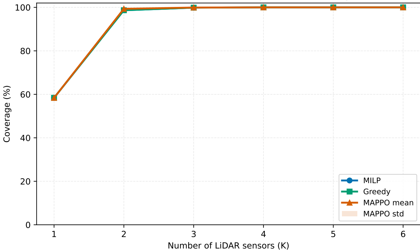
Scenario 0 (STRAIGHT) - Coverage vs. LiDAR Budget
