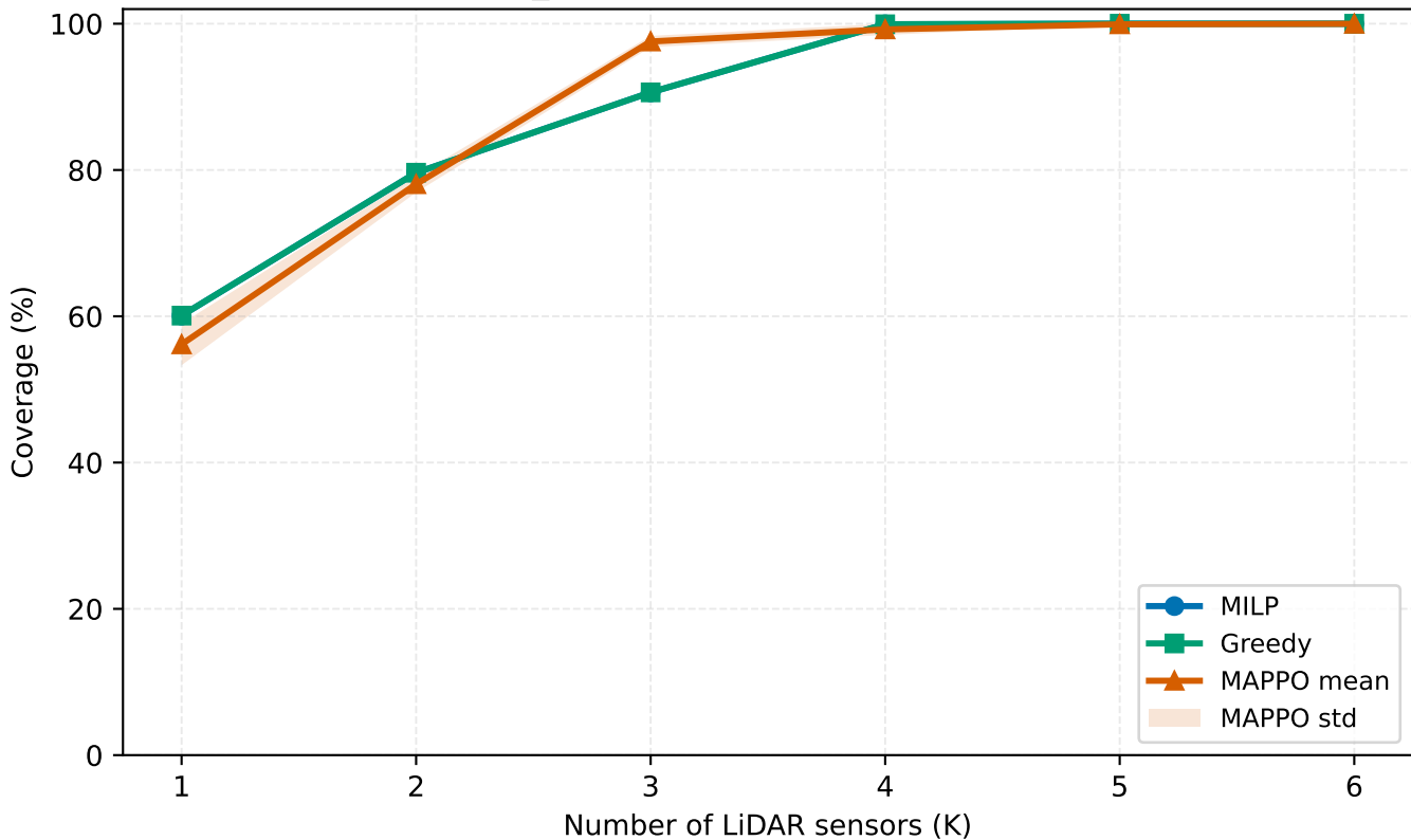
Scenario 1 (T_JUNCTION) - Coverage vs. LiDAR Budget
