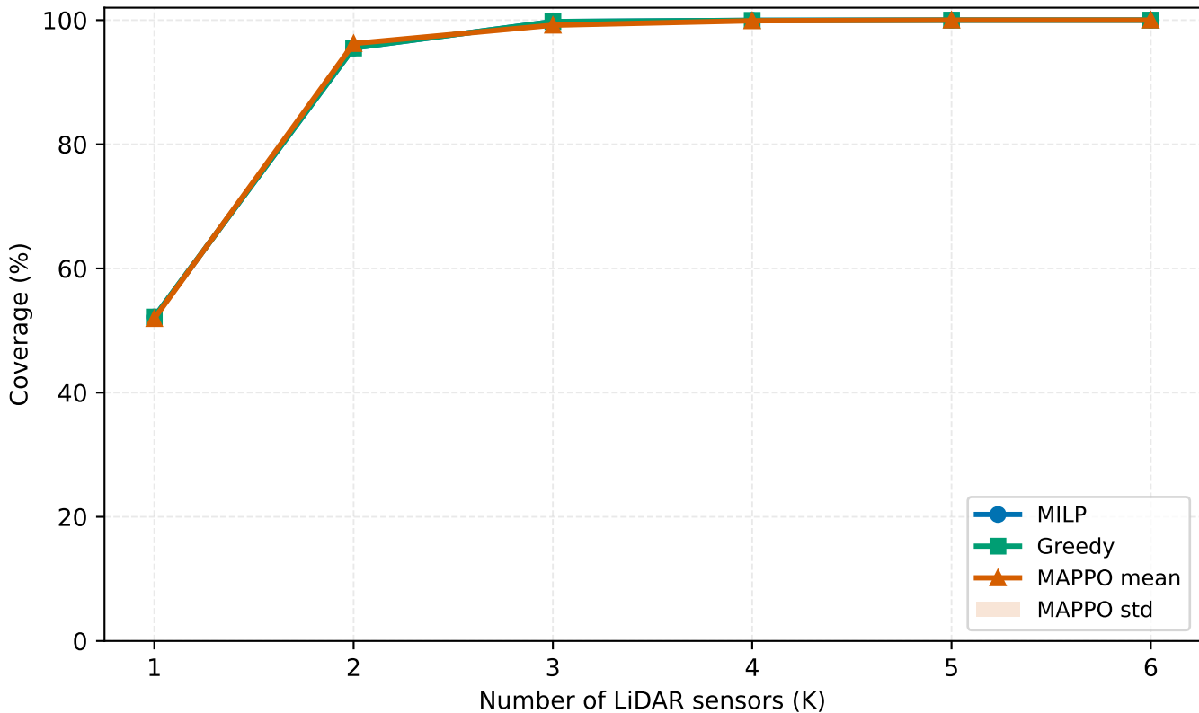
Scenario 3 (STRAIGHT) - Coverage vs. LiDAR Budget
