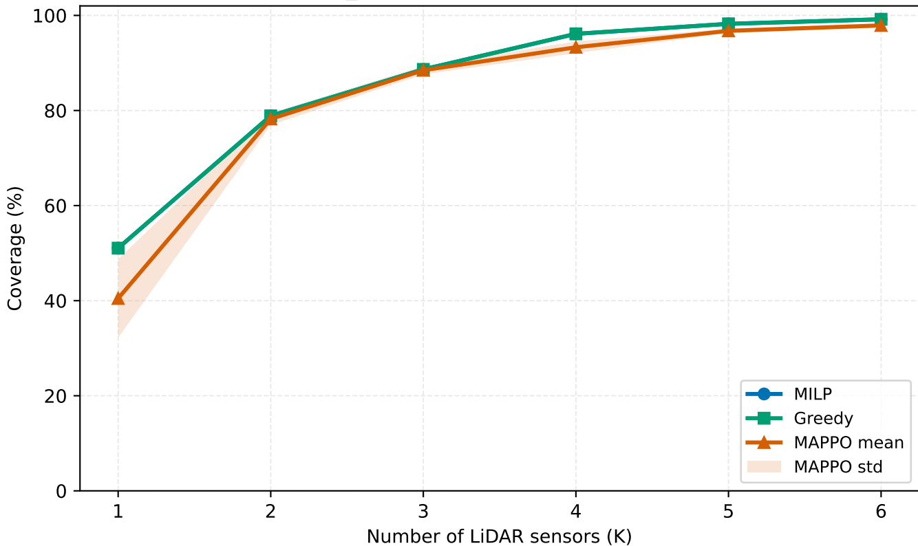
Scenario 9 (T_JUNCTION) - Coverage vs. LiDAR Budget
