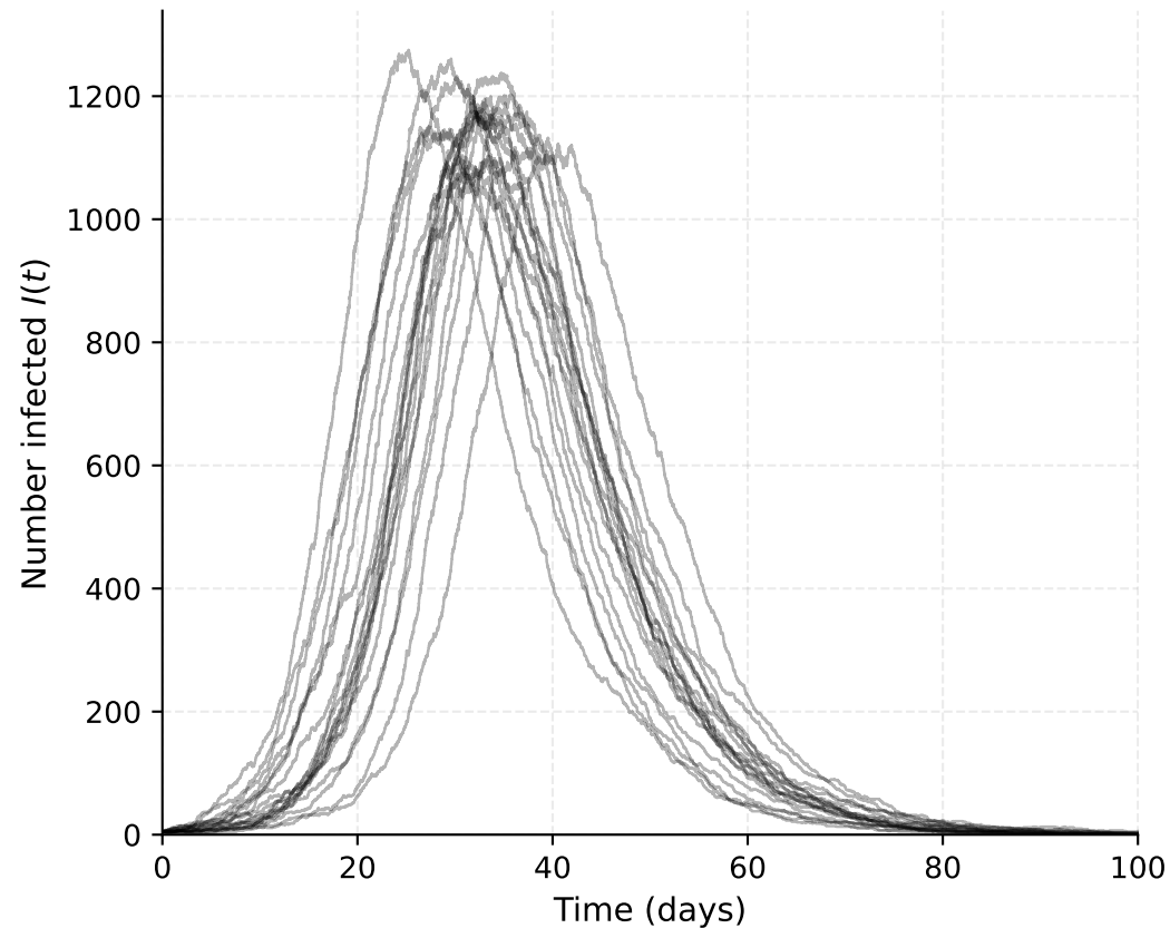
(a) Homogeneous mixing (Gillespie SSA)
