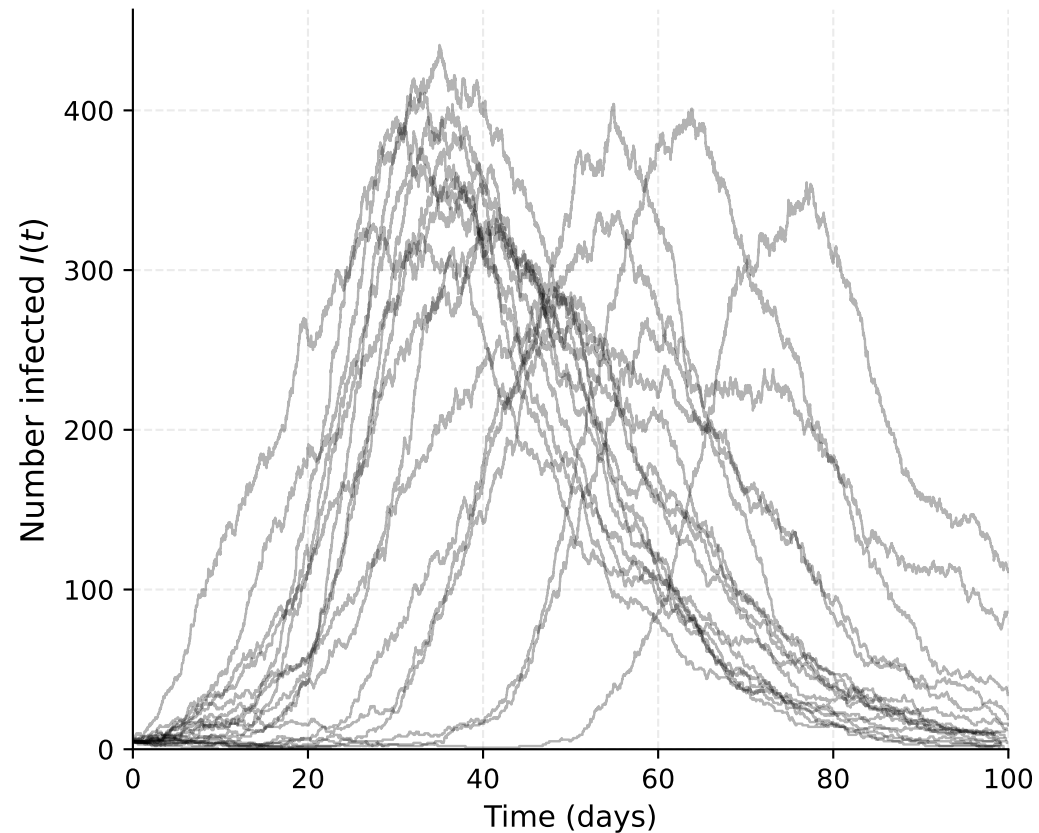
(b) Barabasi-Albert network
