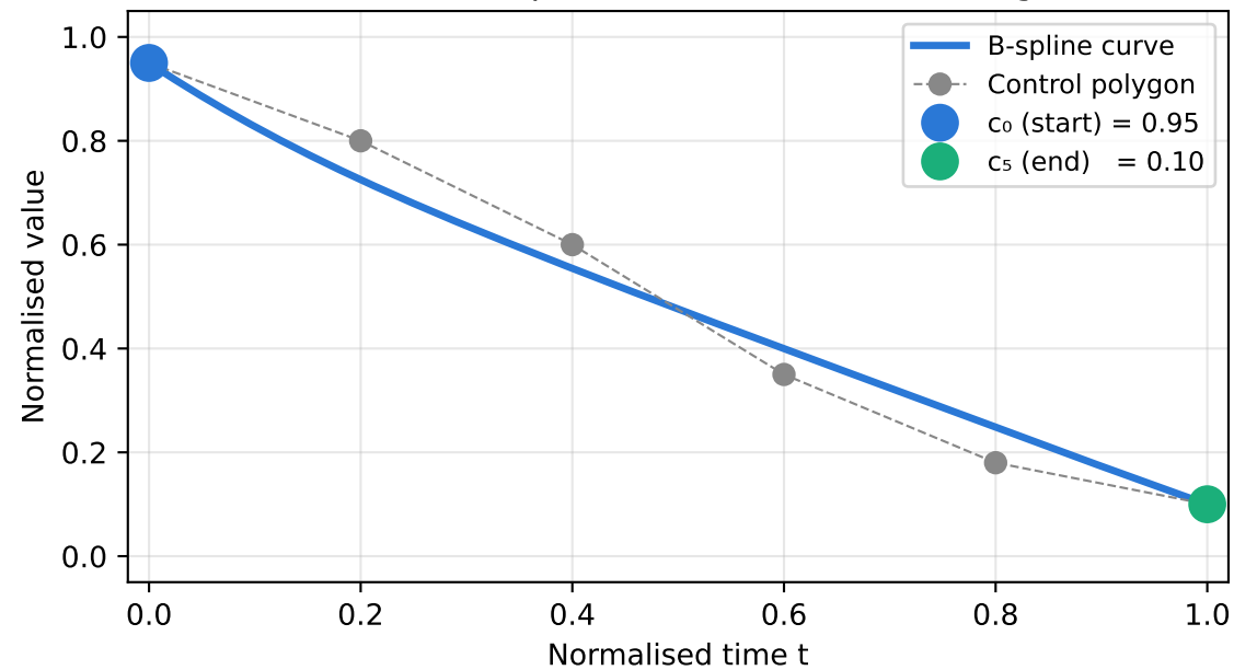
S(t) — Susceptible (monotone decreasing)
