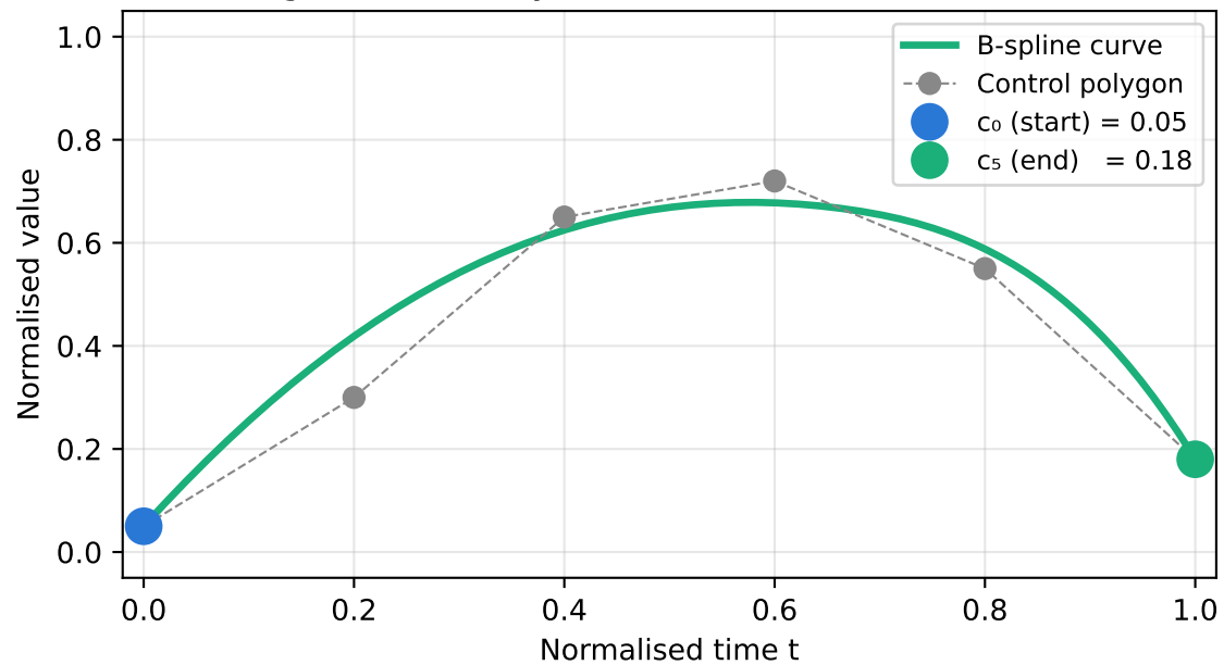
g(t) — Auxiliary function (infectious fraction)
