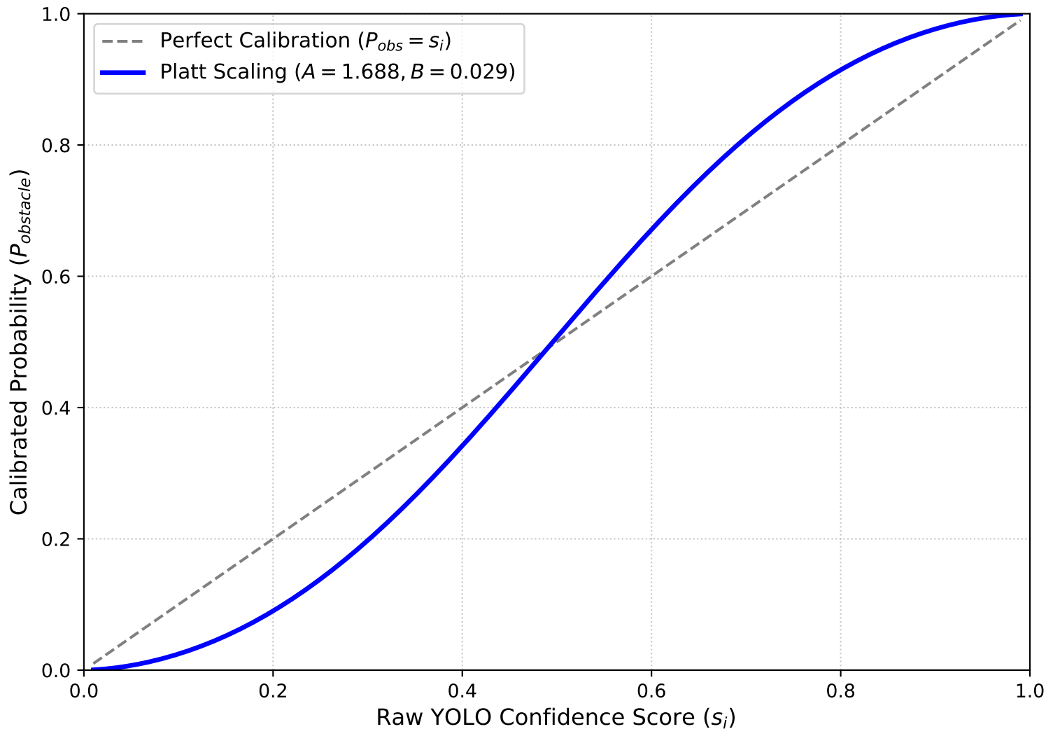
Logistic Sigmoid Function obtained from Platt Scaling calibration method
