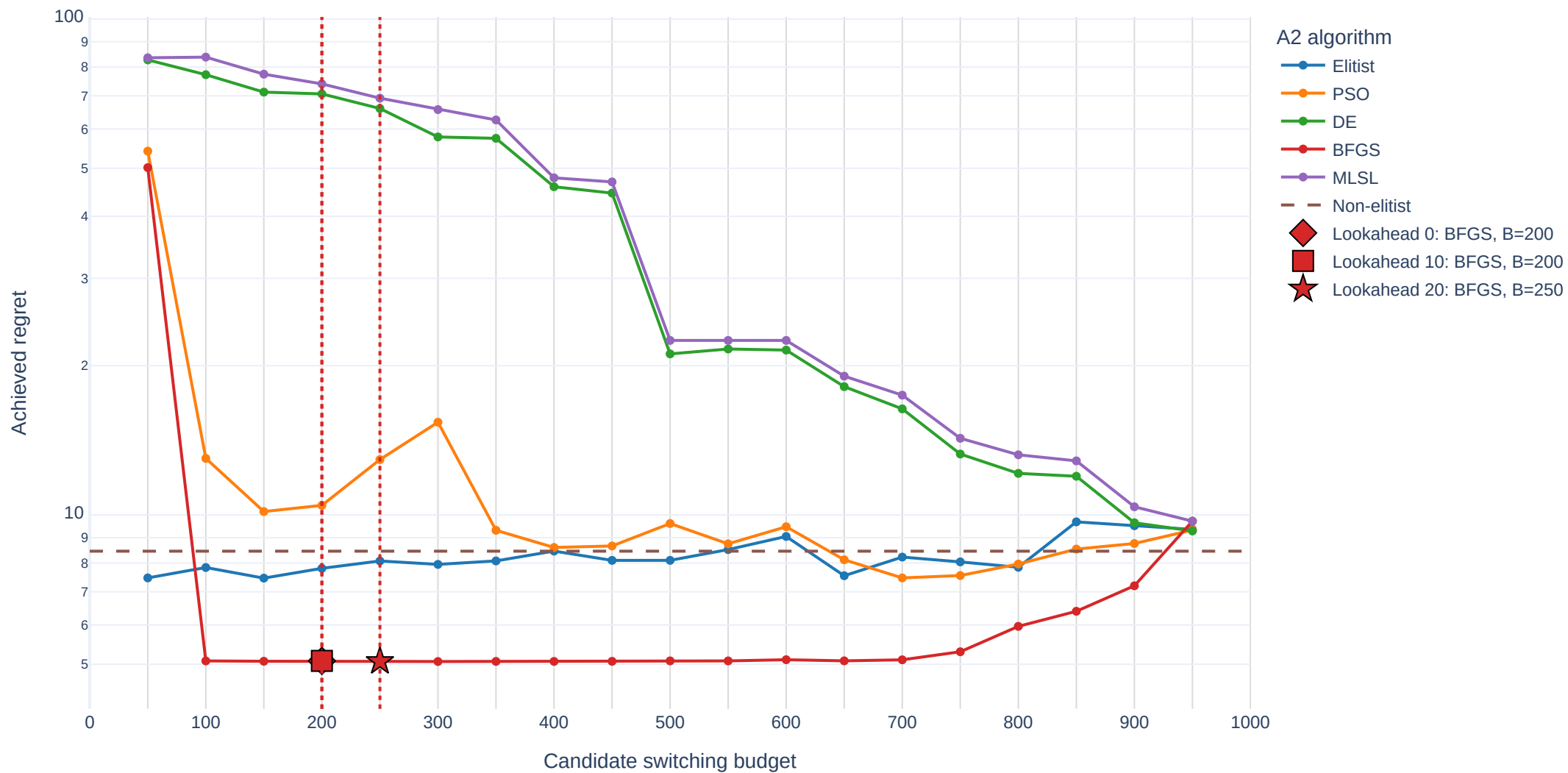
Achieved regret — f22, iid 6, rep 18 (40D)
