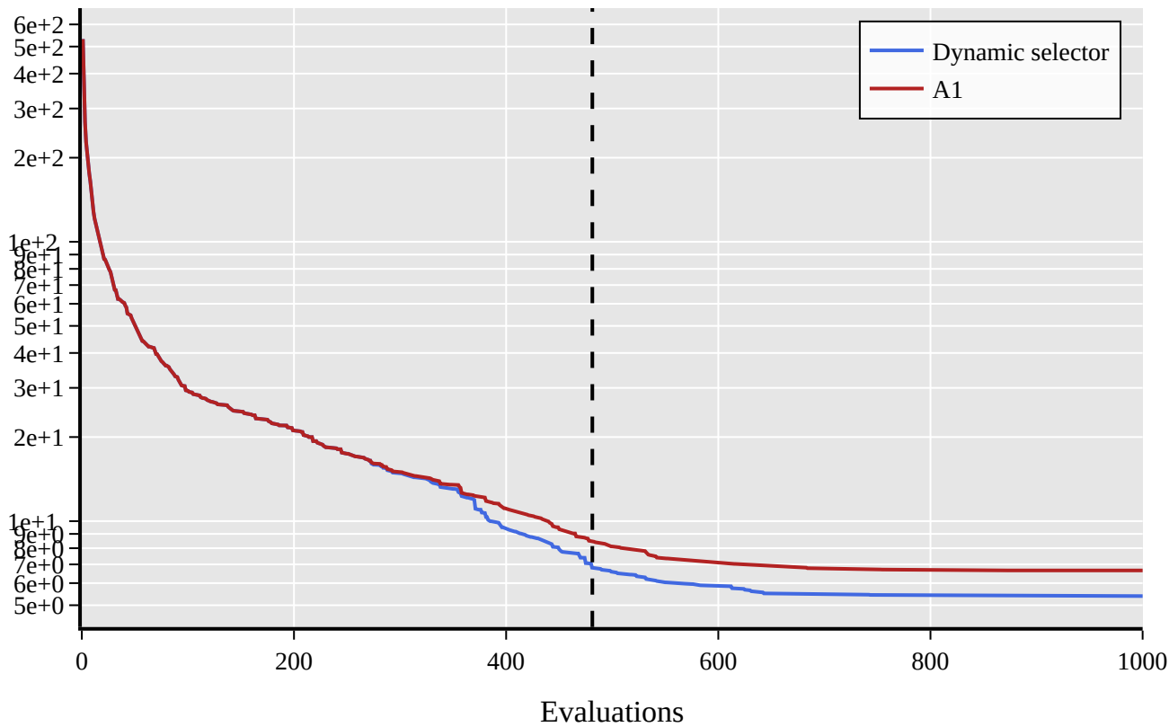
Mean regret
