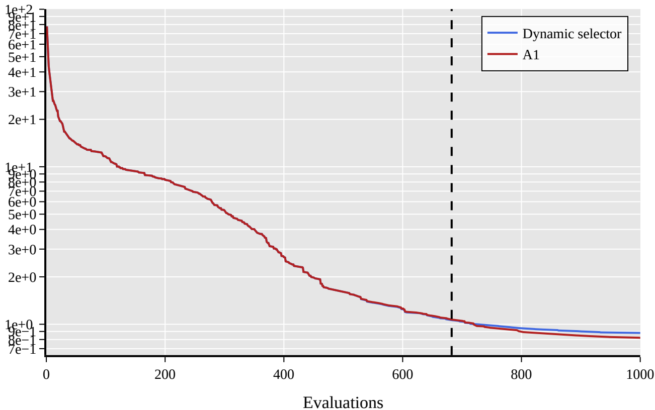
Mean regret
