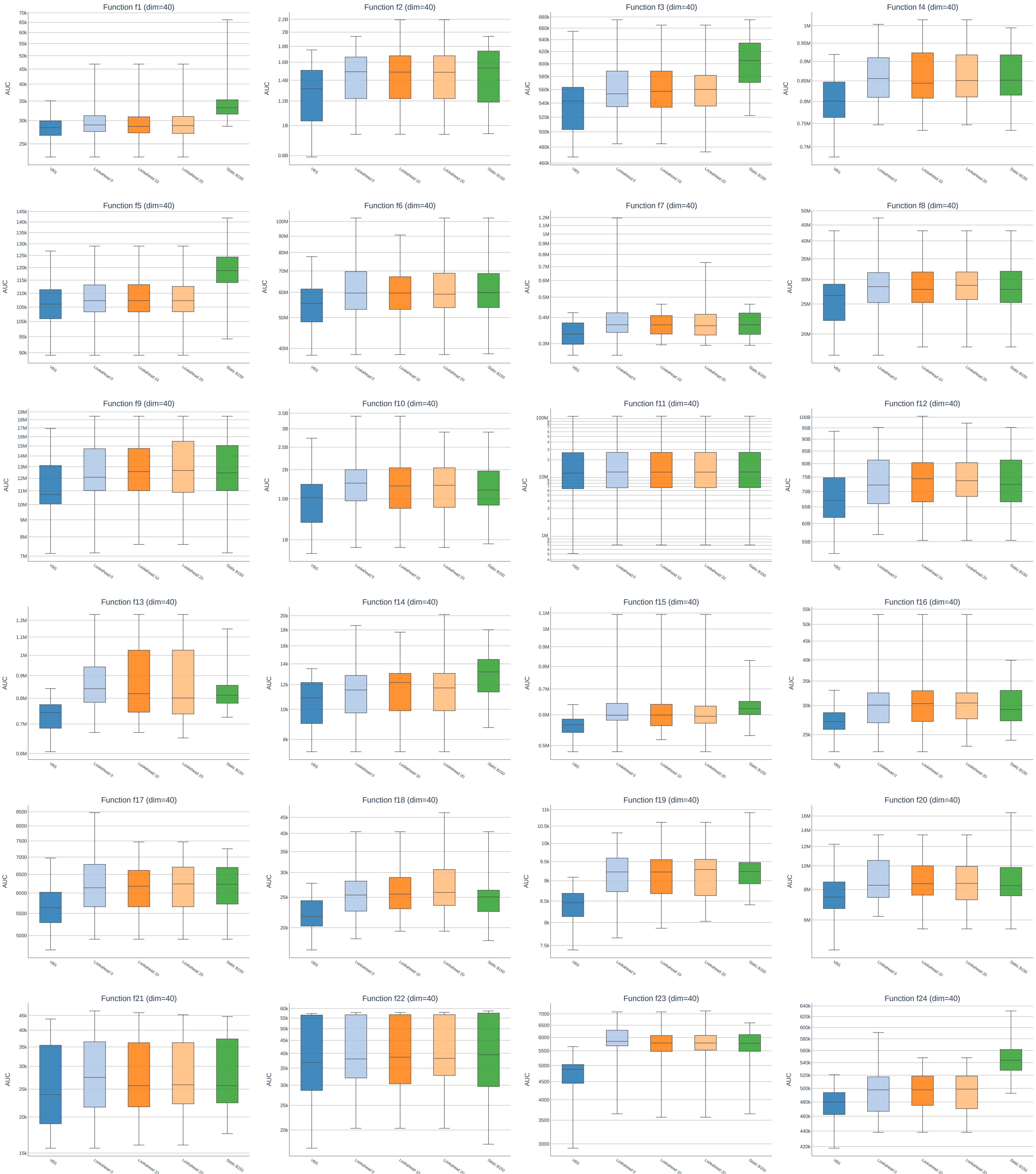
Achieved AUC by BBOB function
