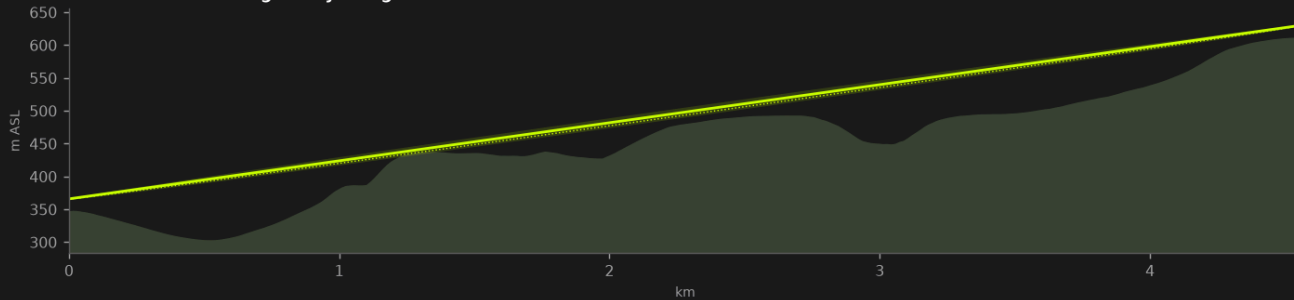
Great Fish River Lodge relay → High Site North 4.6 km · Fresnel zone clear
