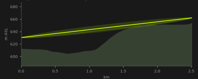
High Site North → North ridge farmstead 2.5 km · Fresnel zone clear
