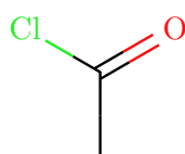
acetyl-chloride
