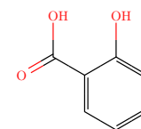
Salicylic
