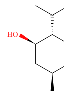
testosterone
