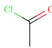
acetyl-chloride
