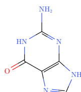
glycine
