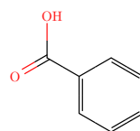
Benzoic
