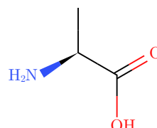
alanine
