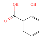
Salicylic
