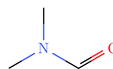
dimethylformamide
