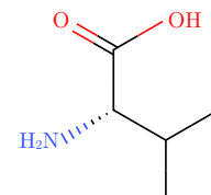
valine
