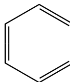
benzaldehyde
