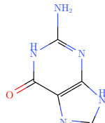
glycine
