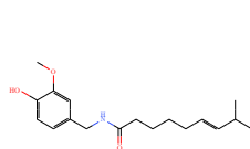
capsaicin
