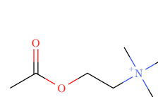
acetylcholine
