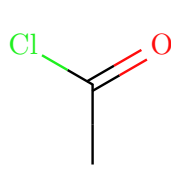
acetyl-chloride
