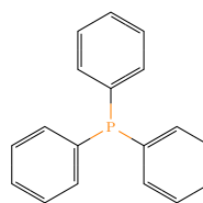
triphenylphosphine
