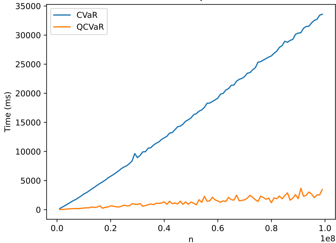
CVaR vs QCVaR
